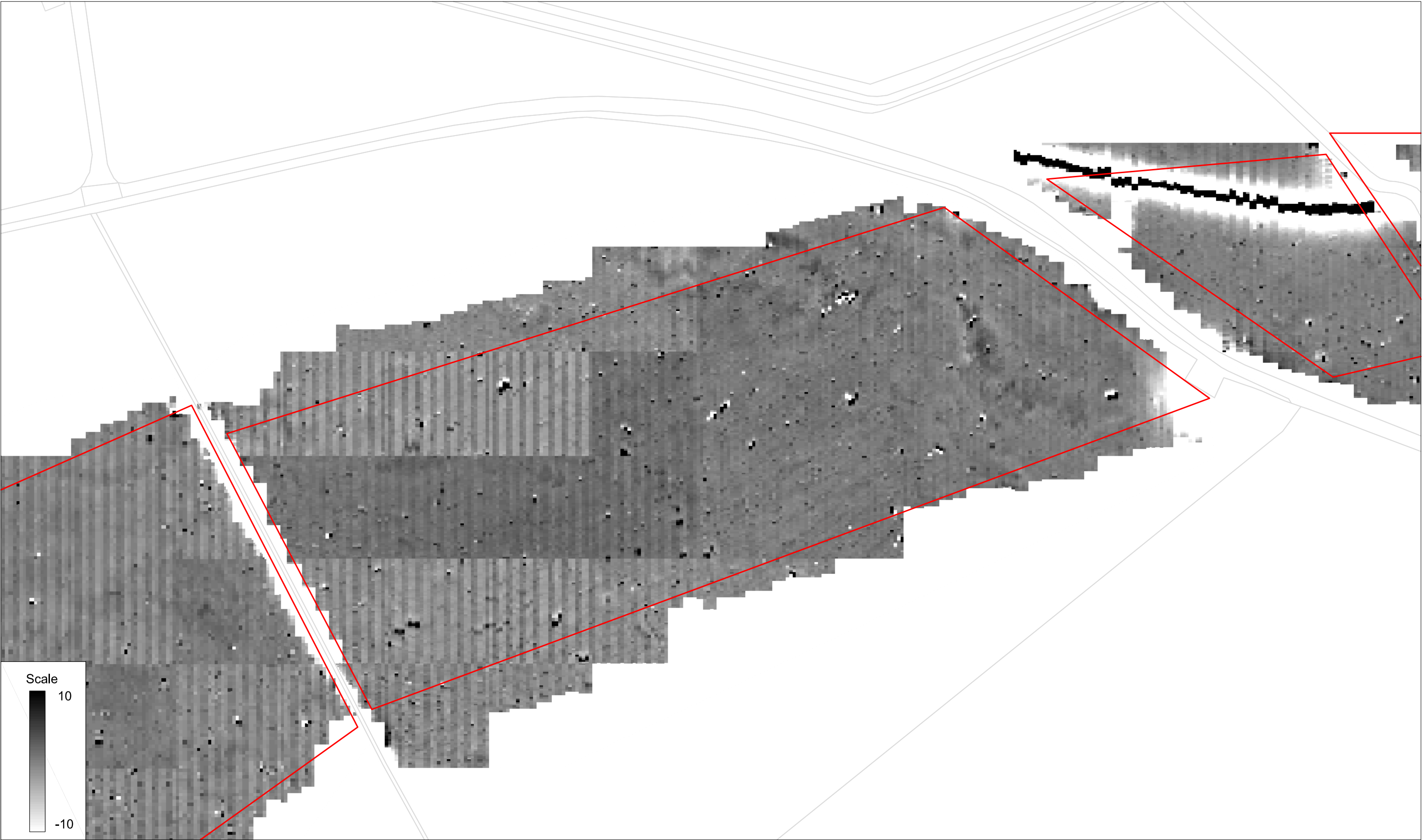
Unprocessed gradiometer survey results greyscale plot: parcel 15c
