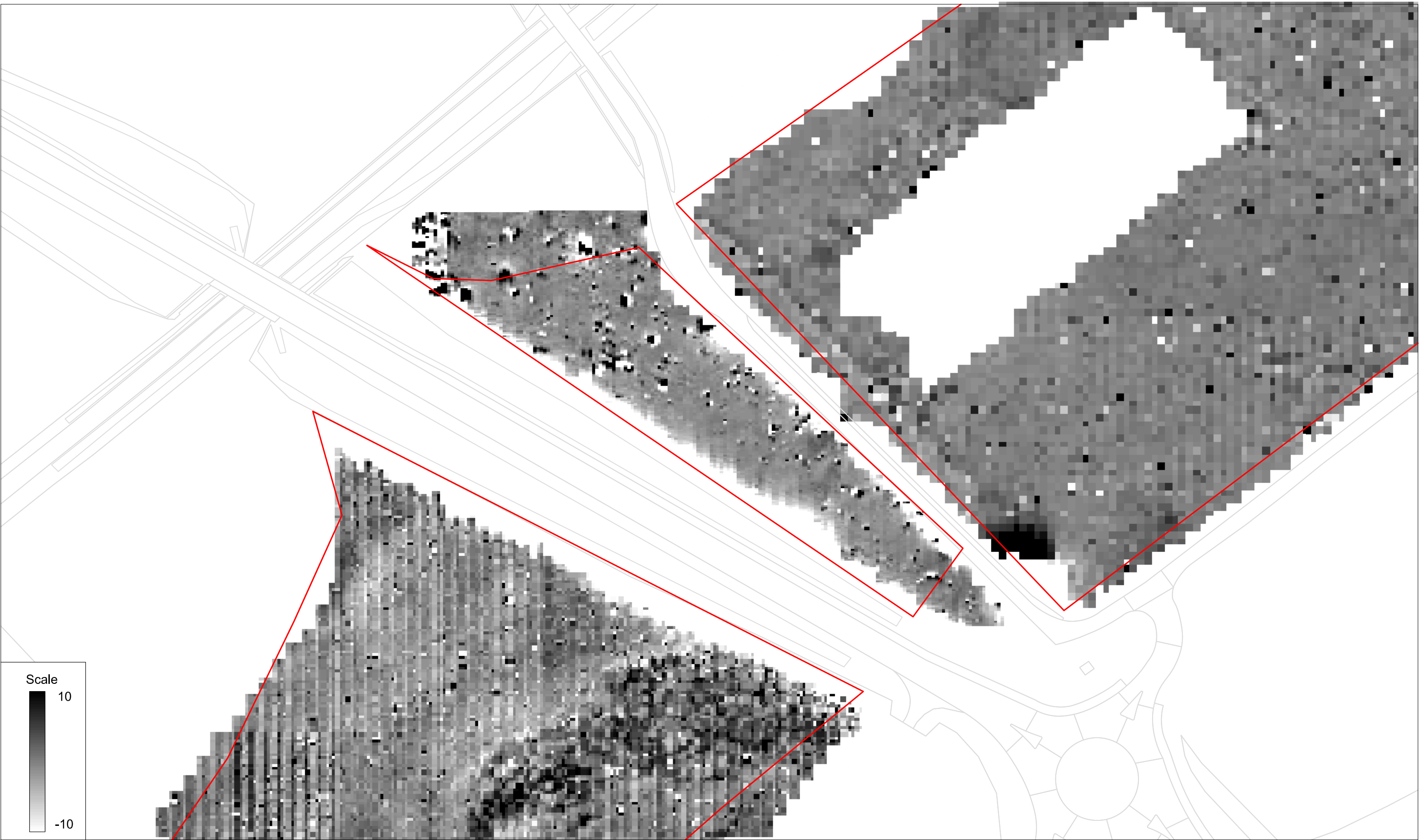
Unprocessed gradiometer survey results greyscale plot: parcel 8c, 8b and 8a
