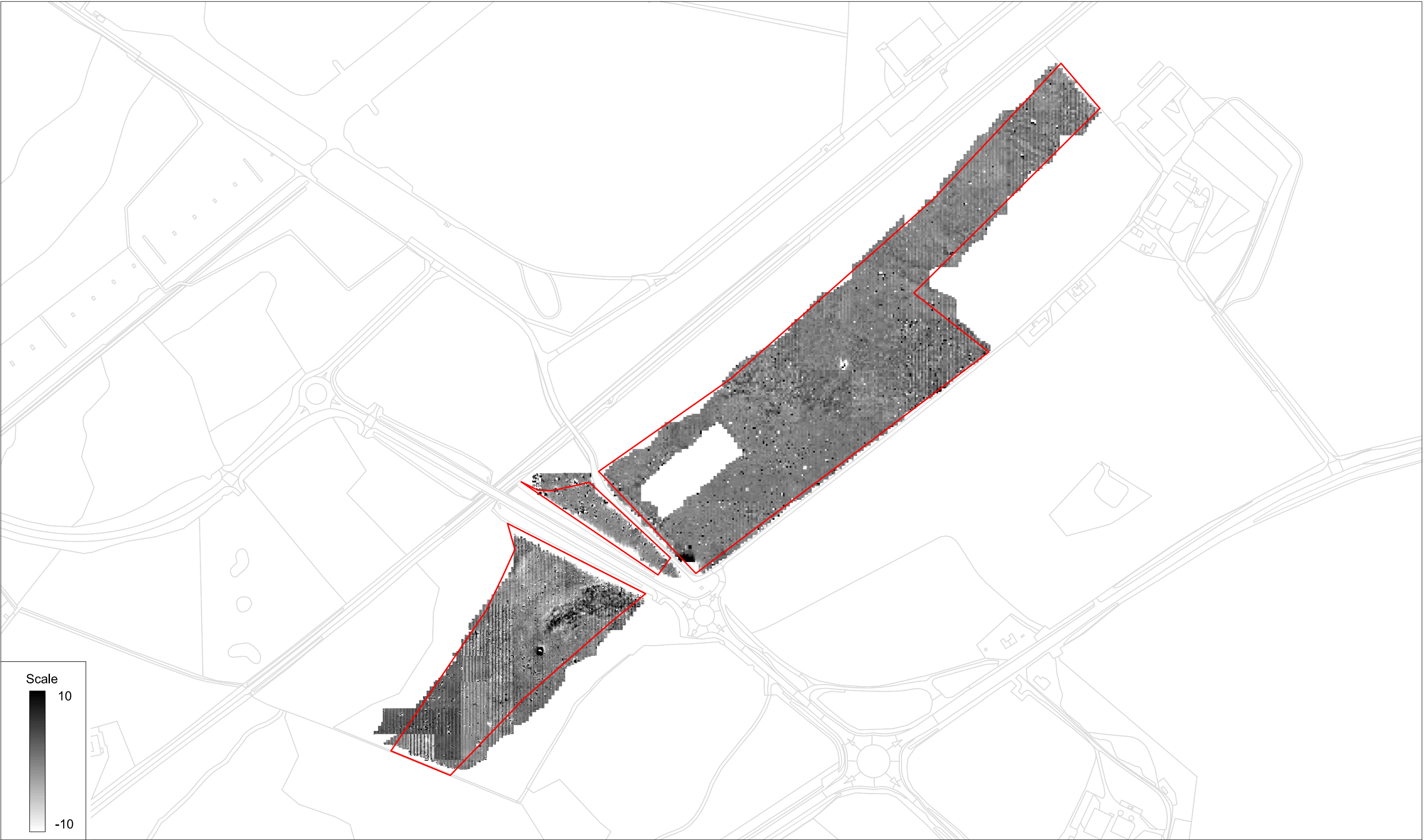
Unprocessed gradiometer survey results greyscale plot: parcel 8
