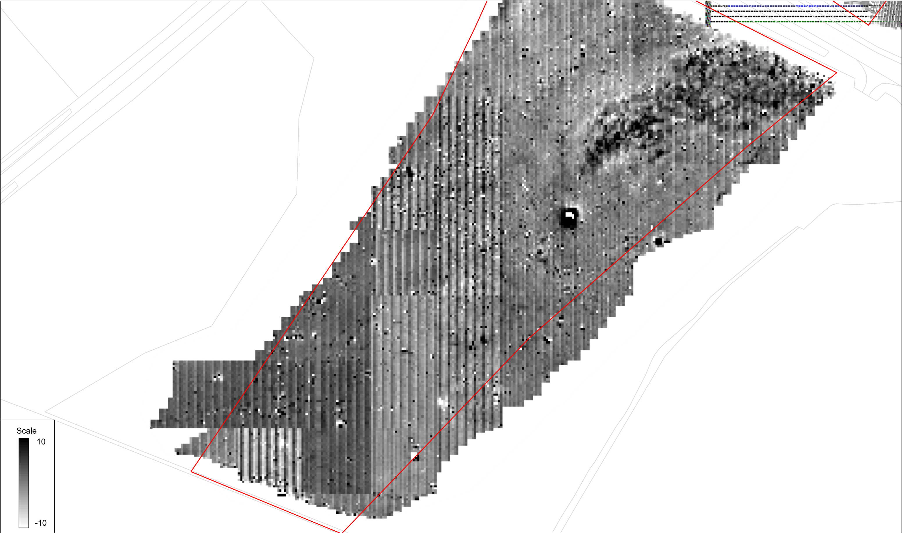
Unprocessed gradiometer survey results greyscale plot: parcel 8c
