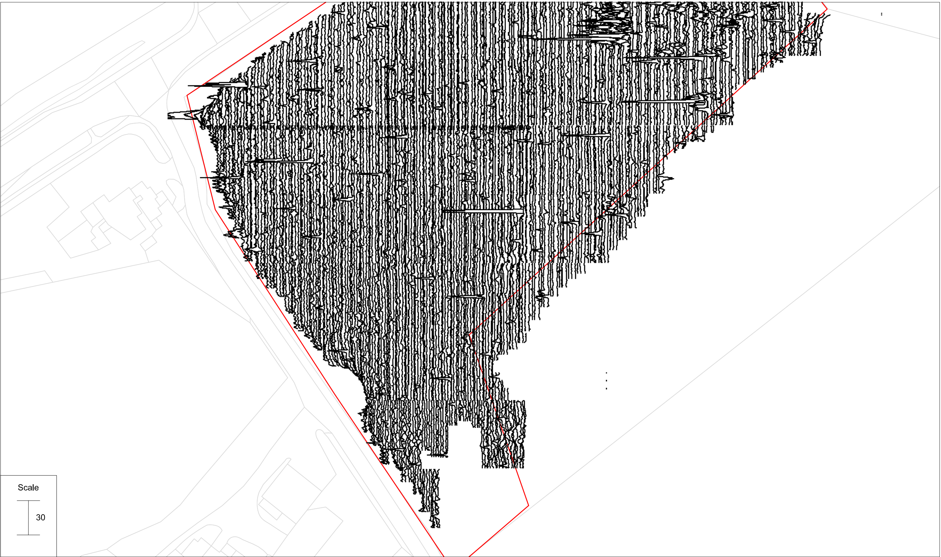
Minimally processed gradiometer survey results xy trace plot: parcel 9a south
