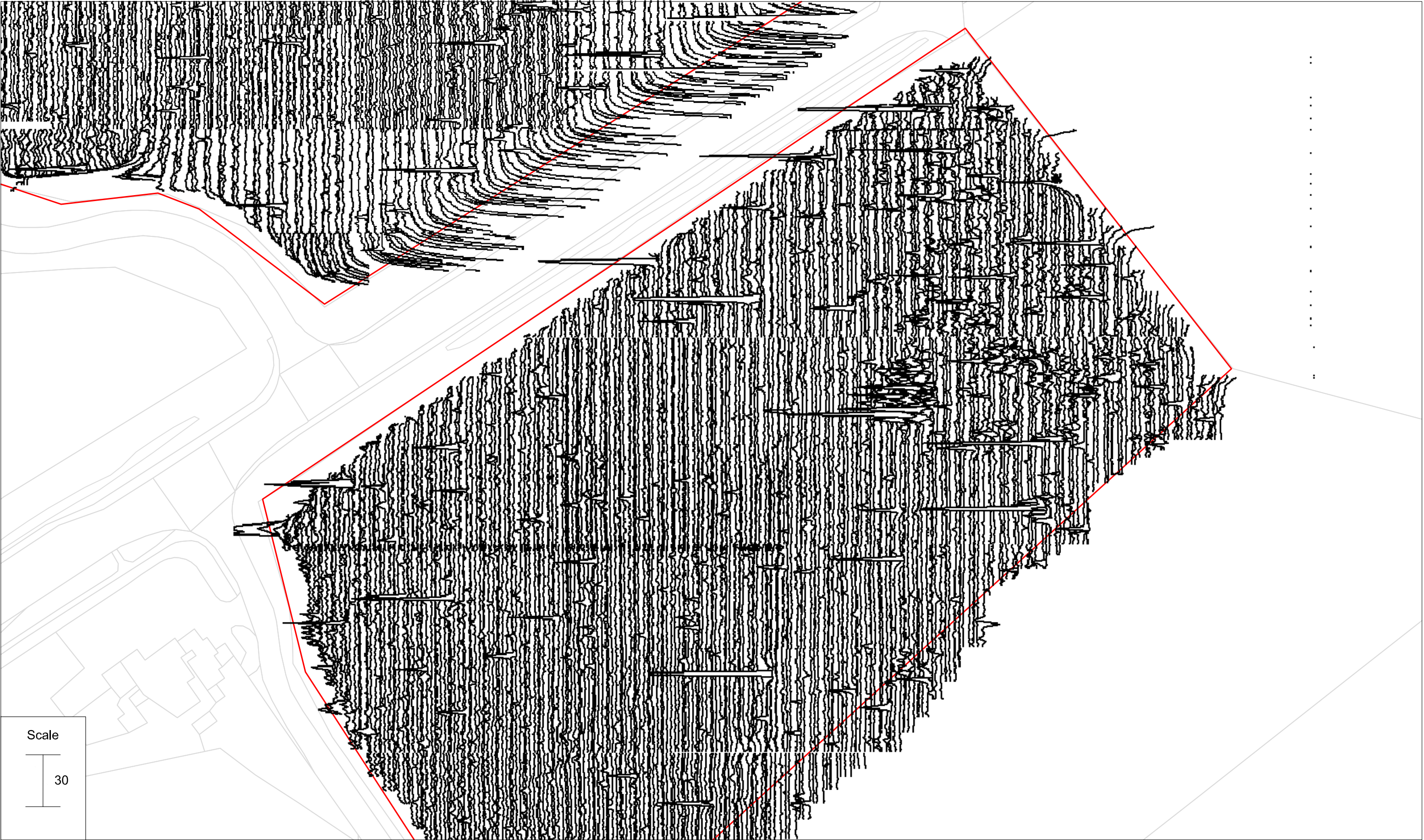
Minimally processed gradiometer survey results xy trace plot: parcel 9a north
