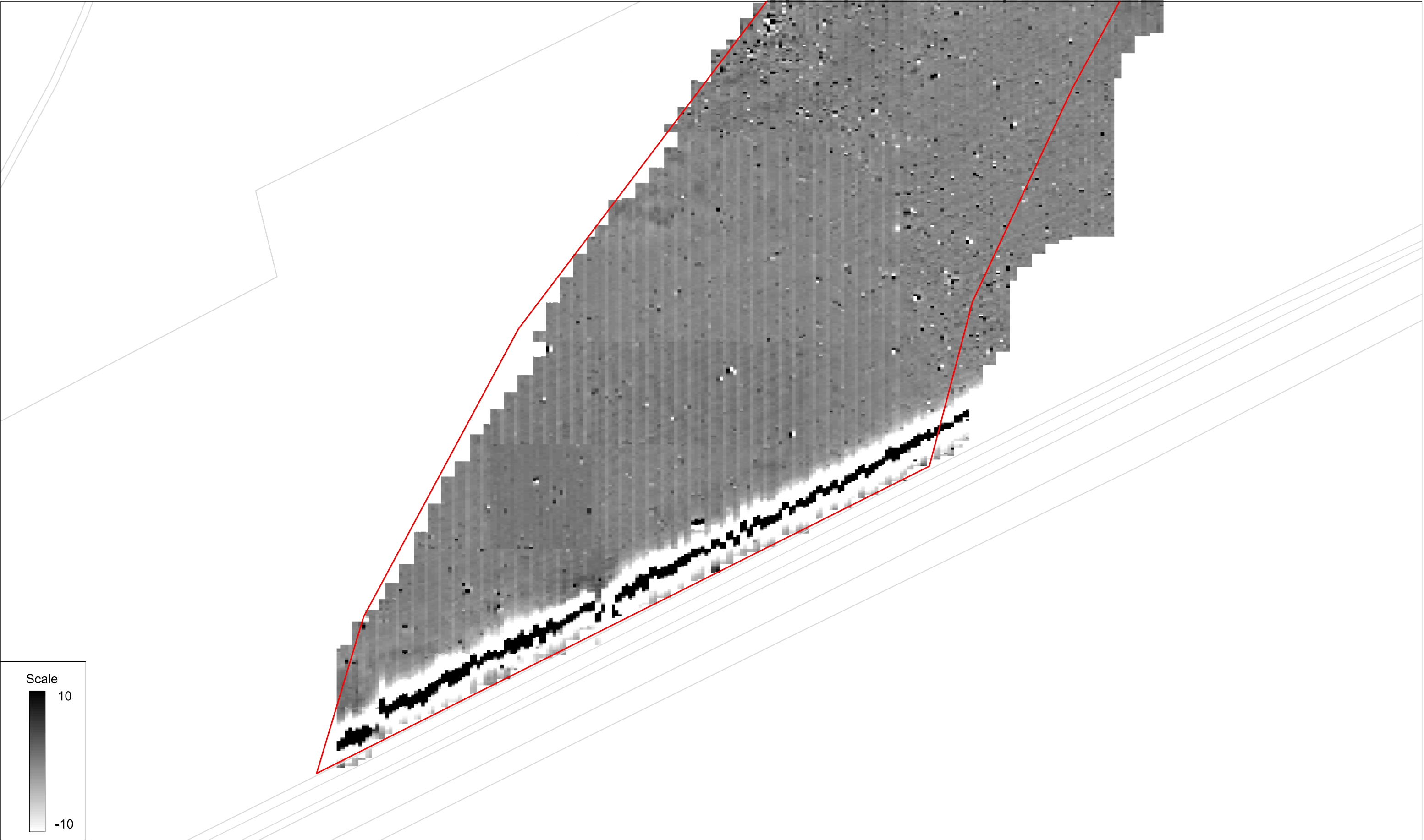
Unprocessed gradiometer survey results greyscale plot: parcel 6 south
