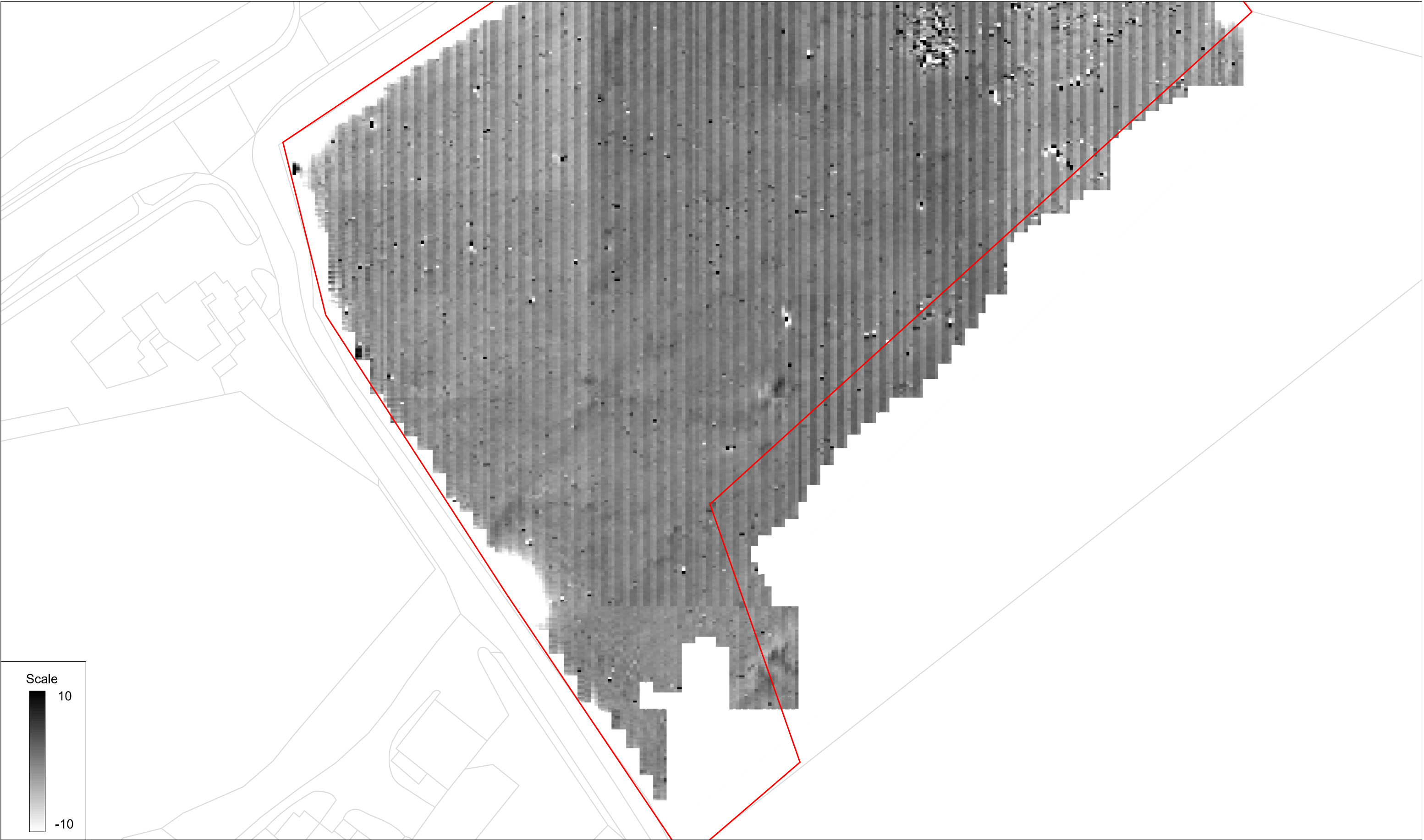
Unprocessed gradiometer survey results greyscale plot: parcel 9a south
