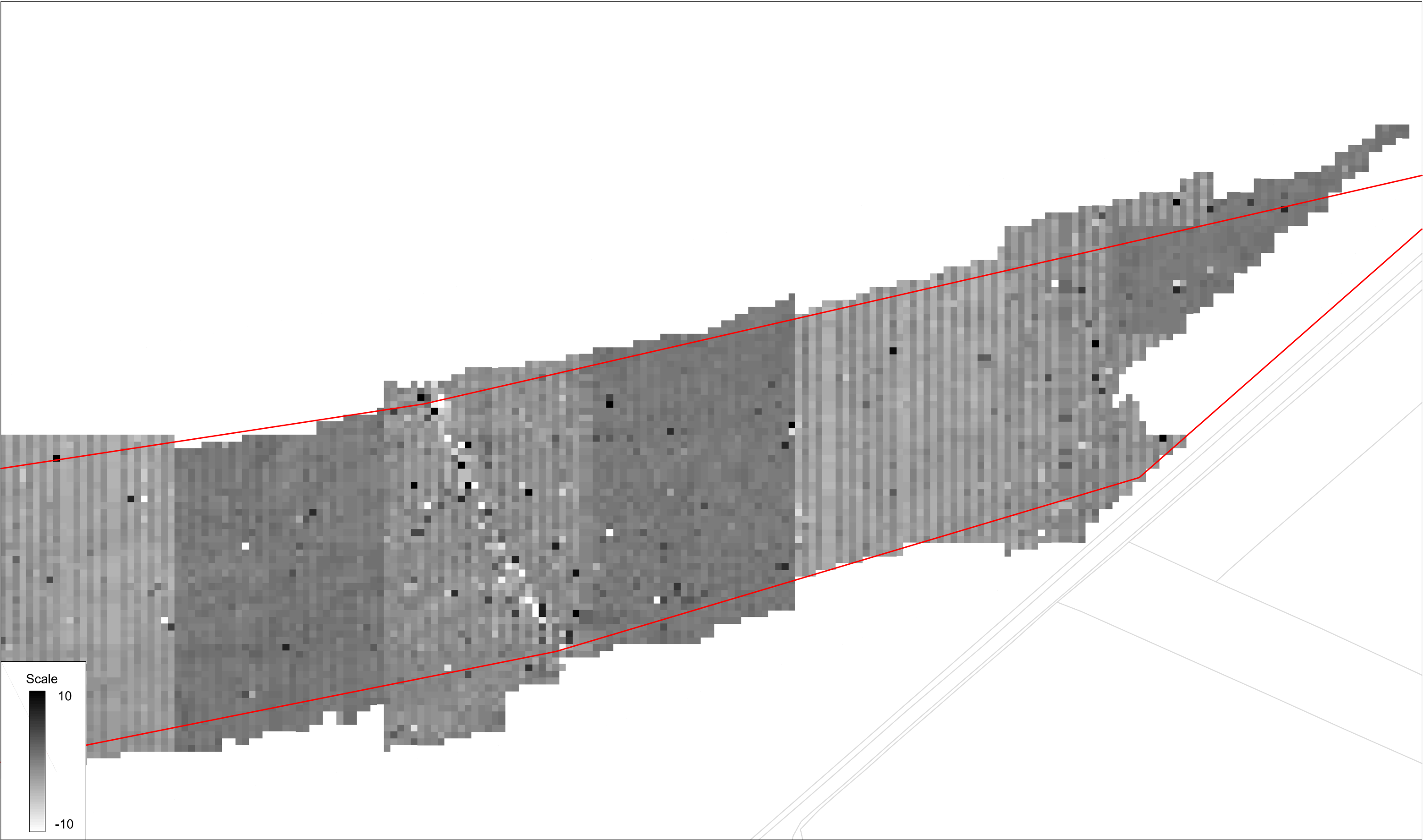
Unprocessed gradiometer survey results greyscale plot: parcel 13a east
