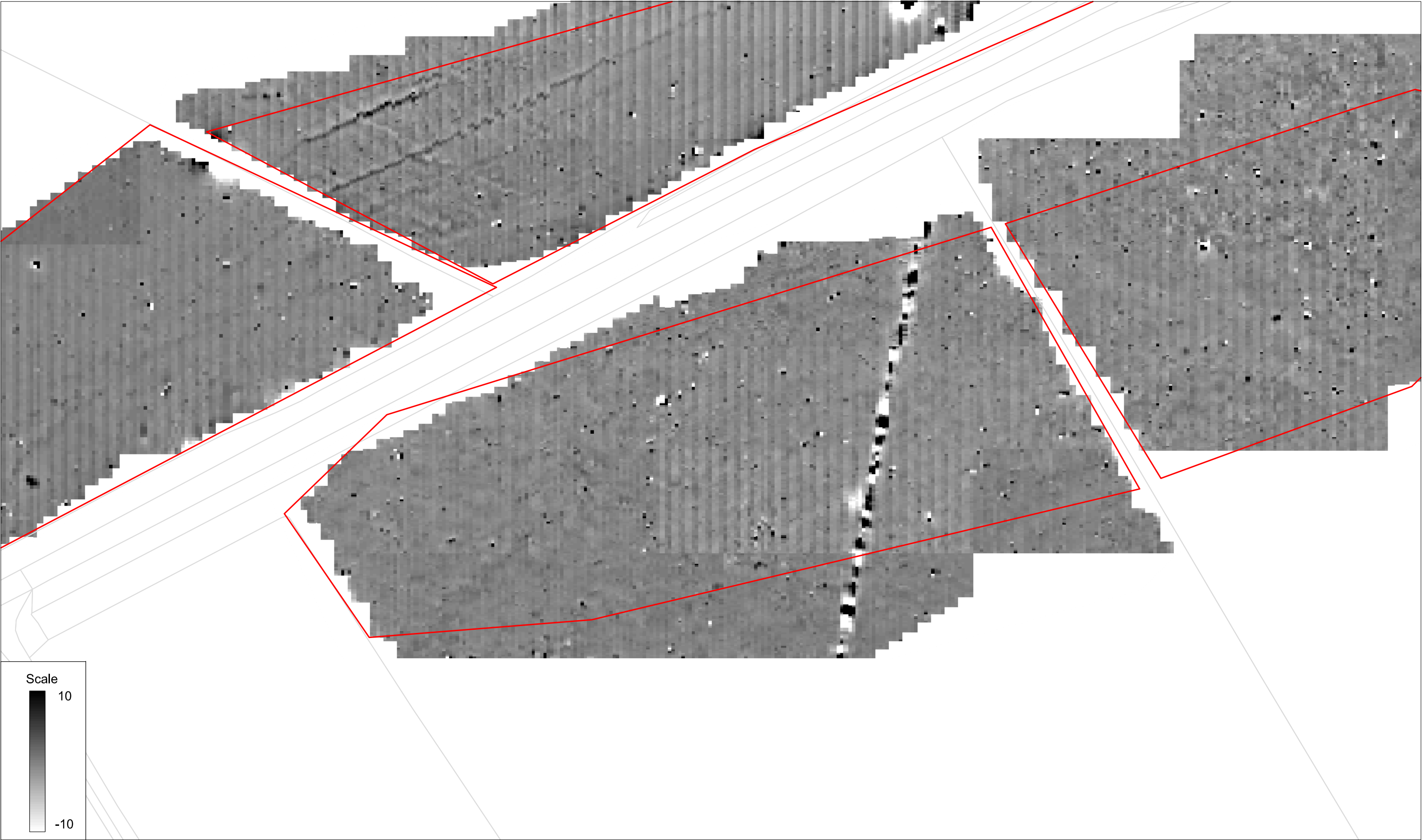
Unprocessed gradiometer survey results greyscale plot: parcel 18a
