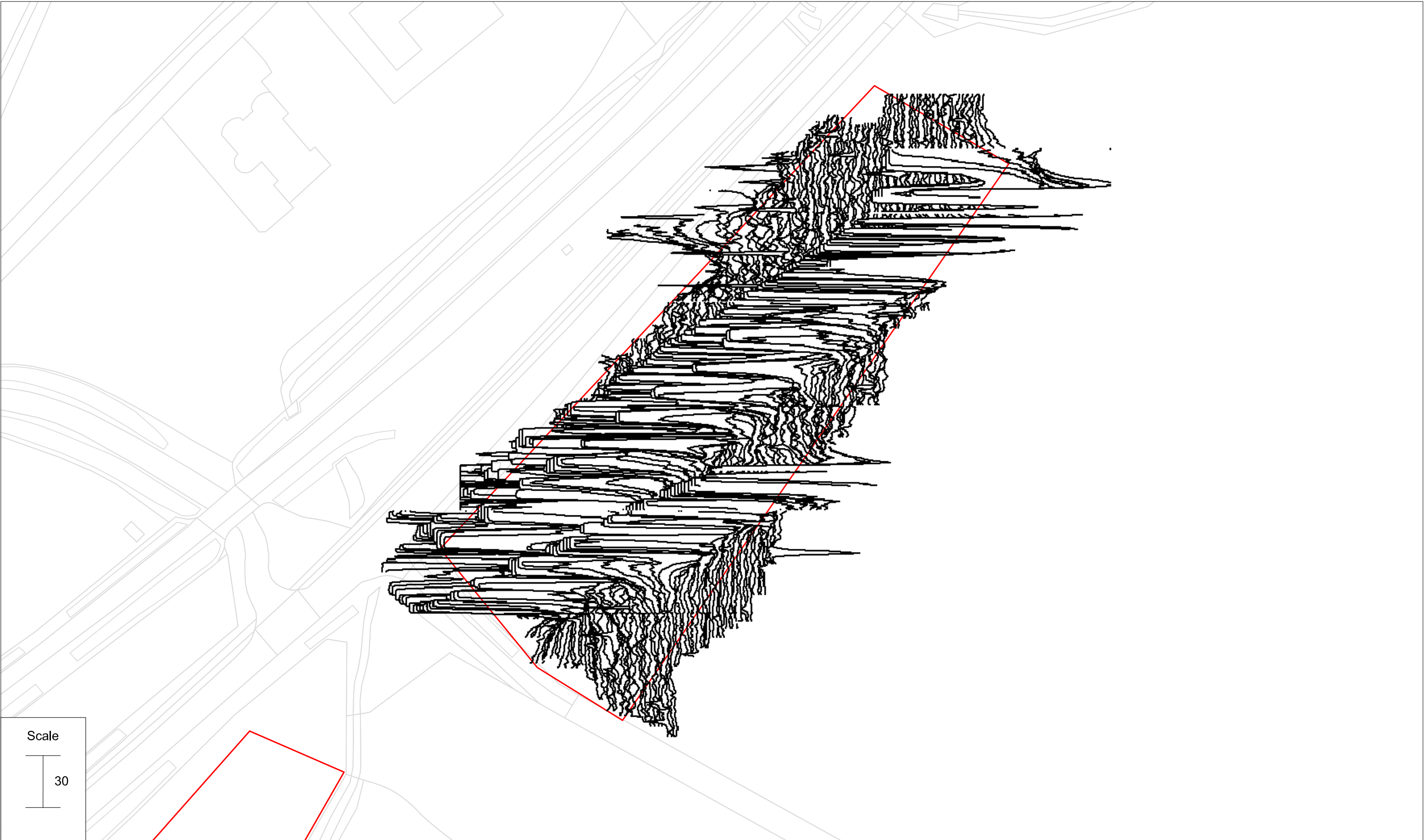
Minimally processed gradiometer survey results xy trace plot: parcel 3
