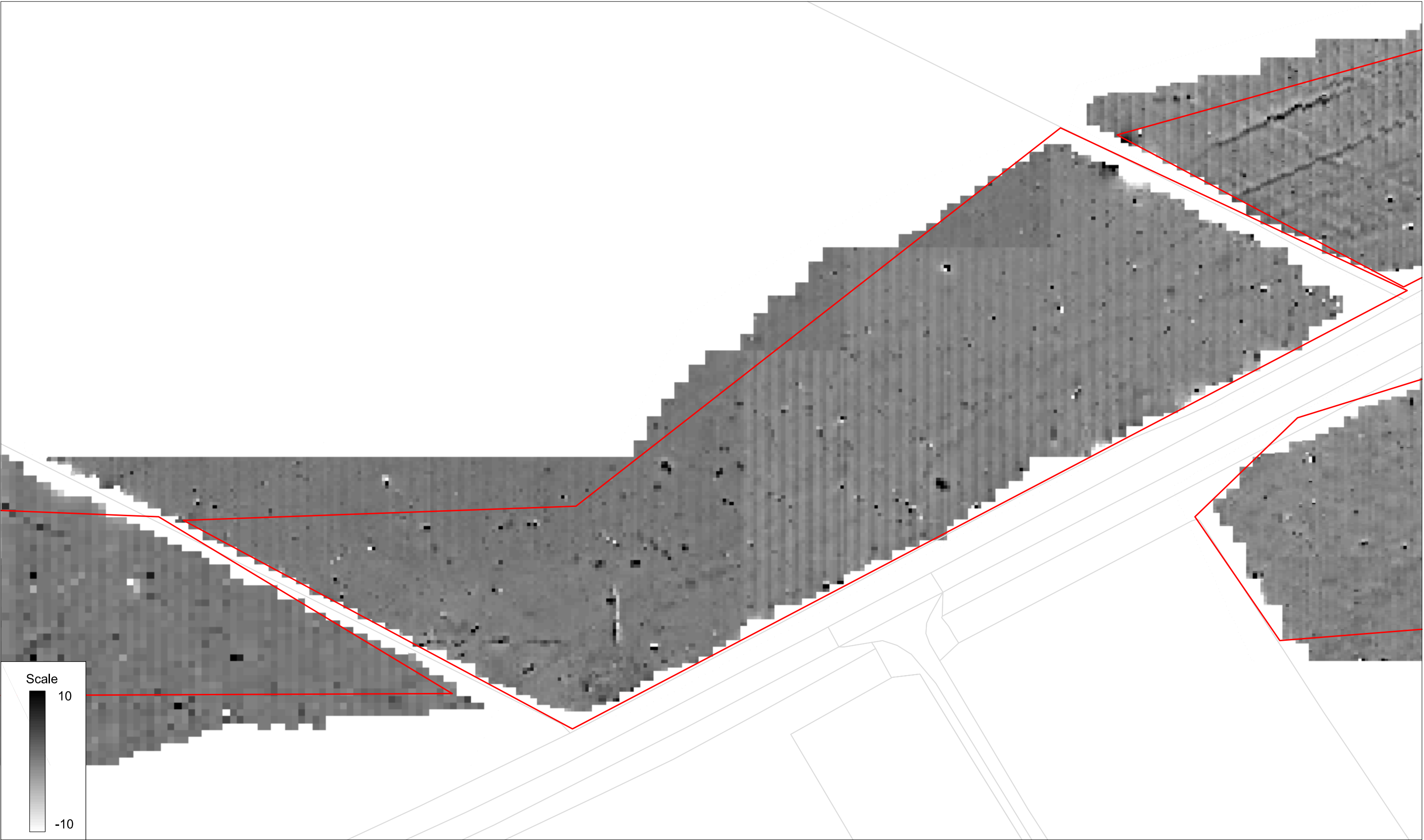
Unprocessed gradiometer survey results greyscale plot: parcel 17b
