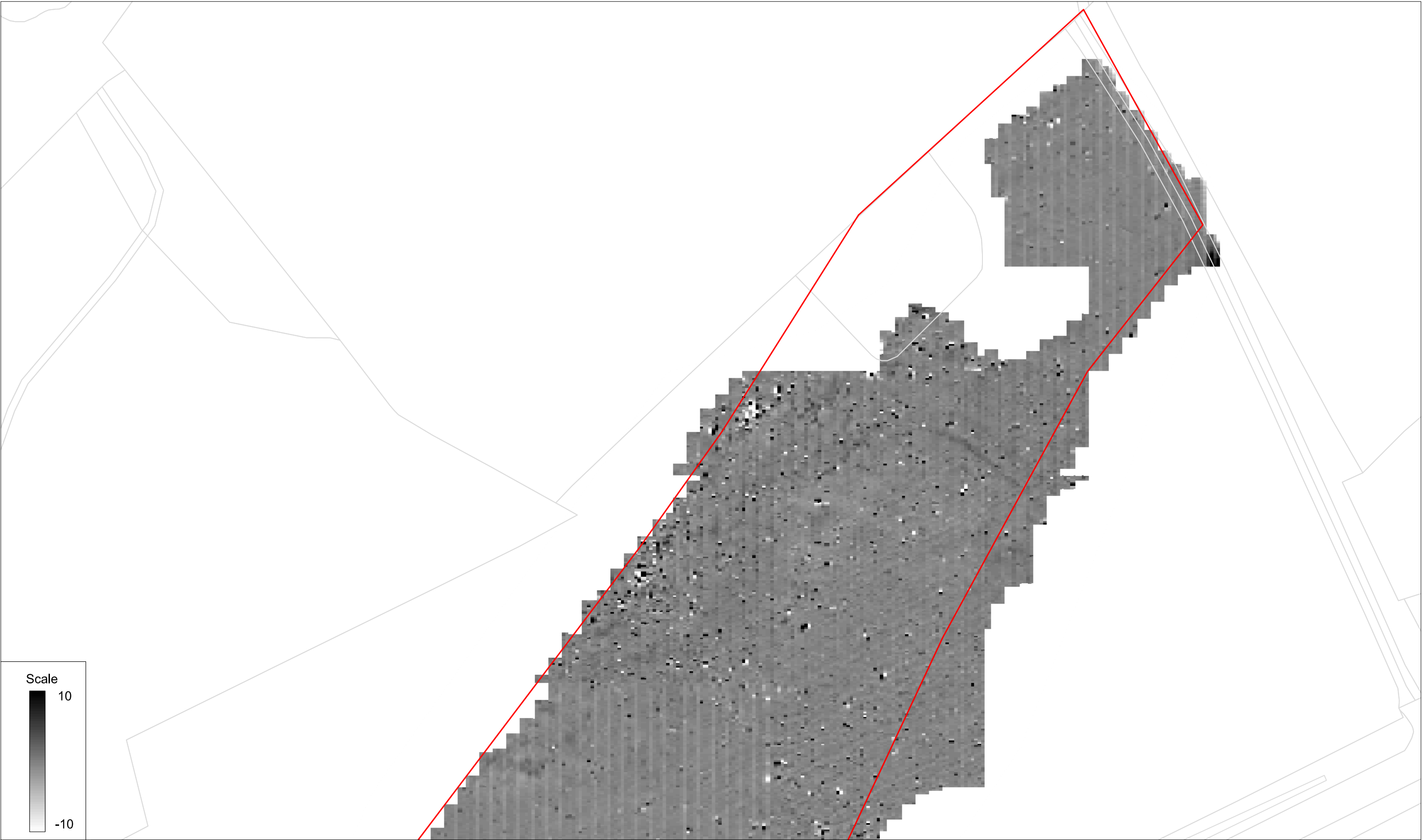
Unprocessed gradiometer survey results greyscale plot: parcel 6 north
