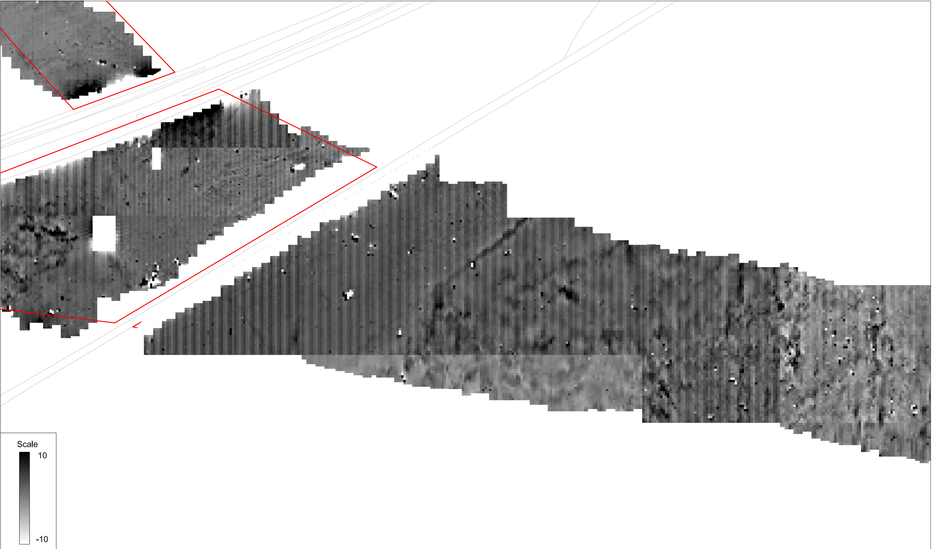
Unprocessed gradiometer survey results greyscale plot: parcel 12c west
