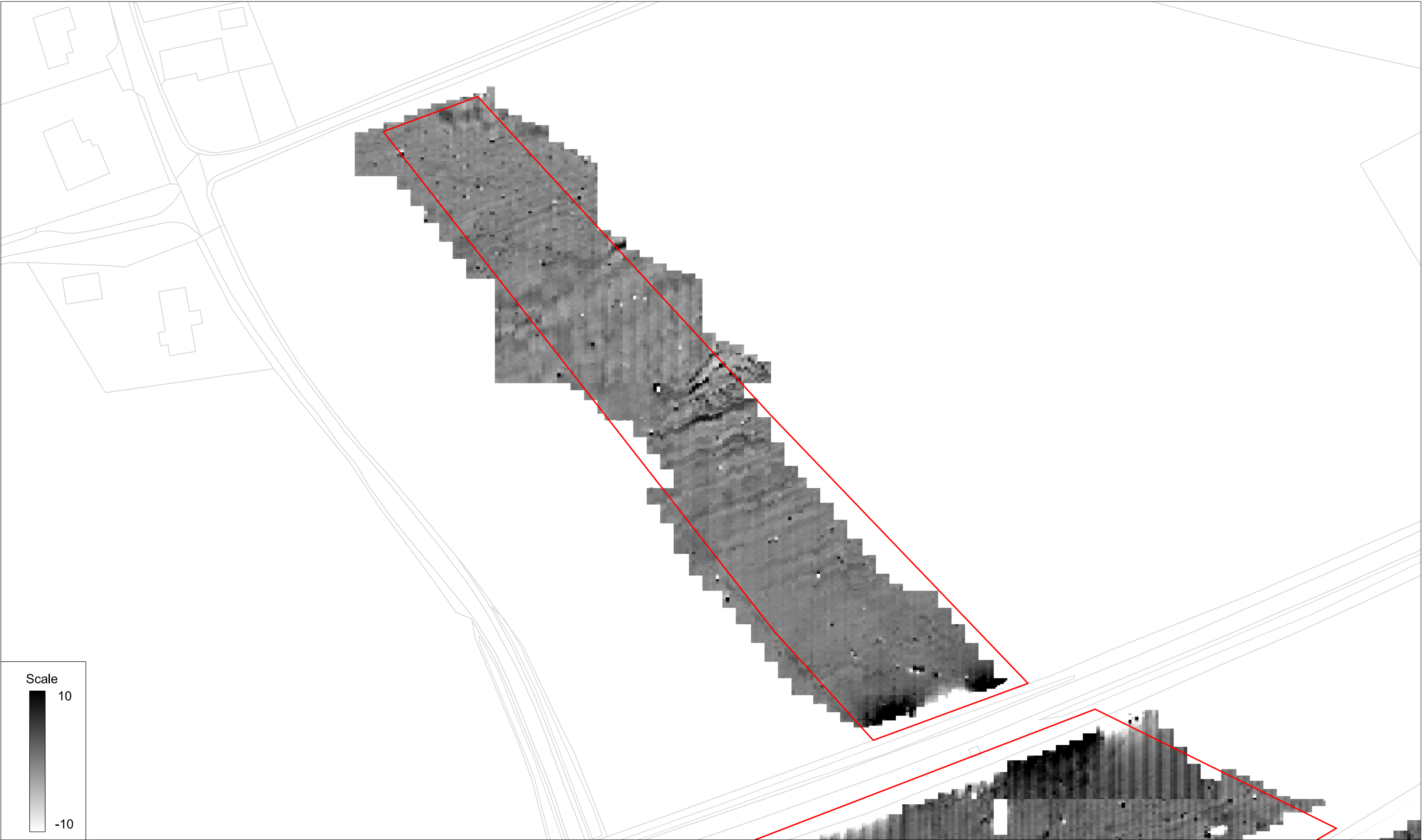
Unprocessed gradiometer survey results greyscale plot: parcel 12a
