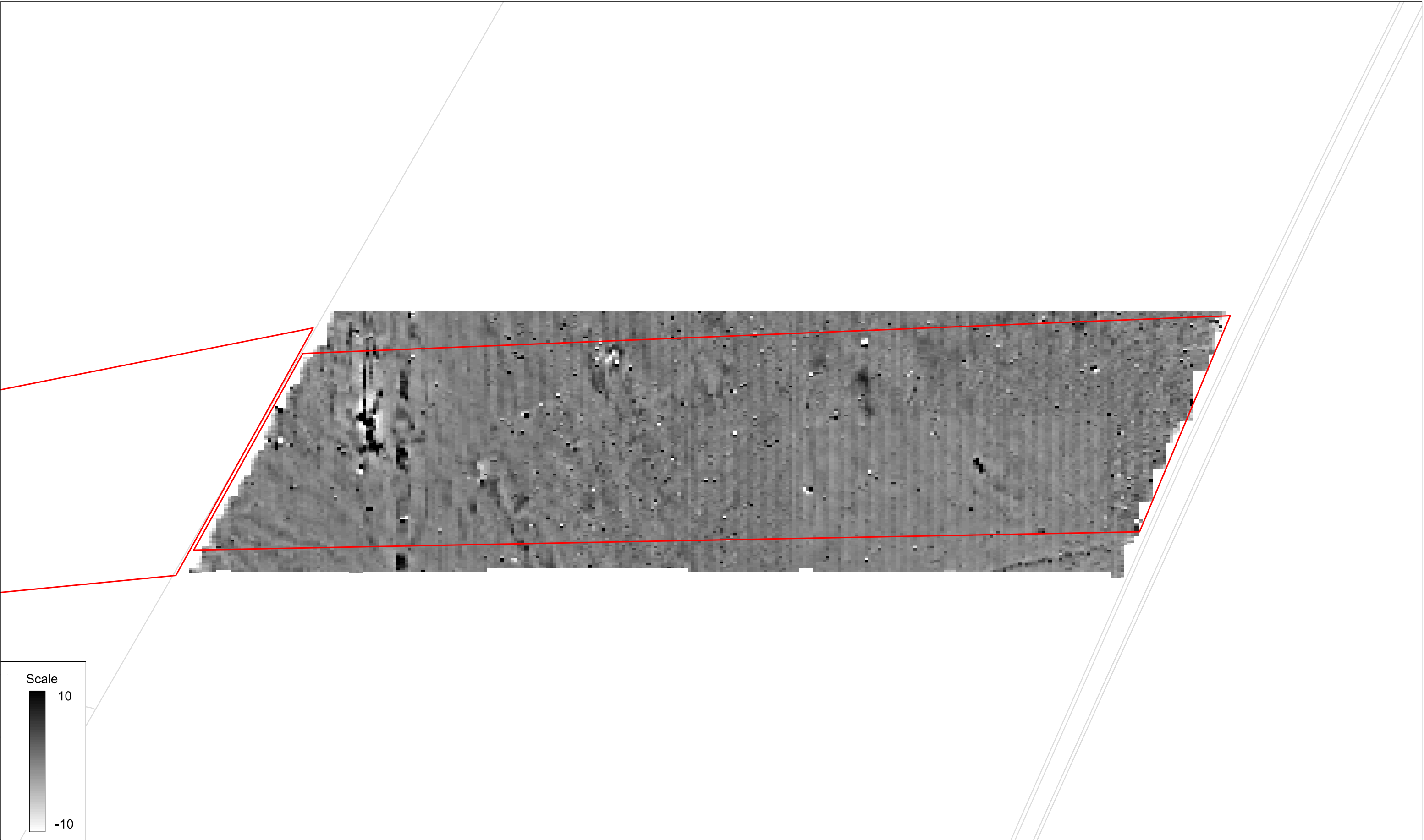
Unprocessed gradiometer survey results greyscale plot: parcel 13b
