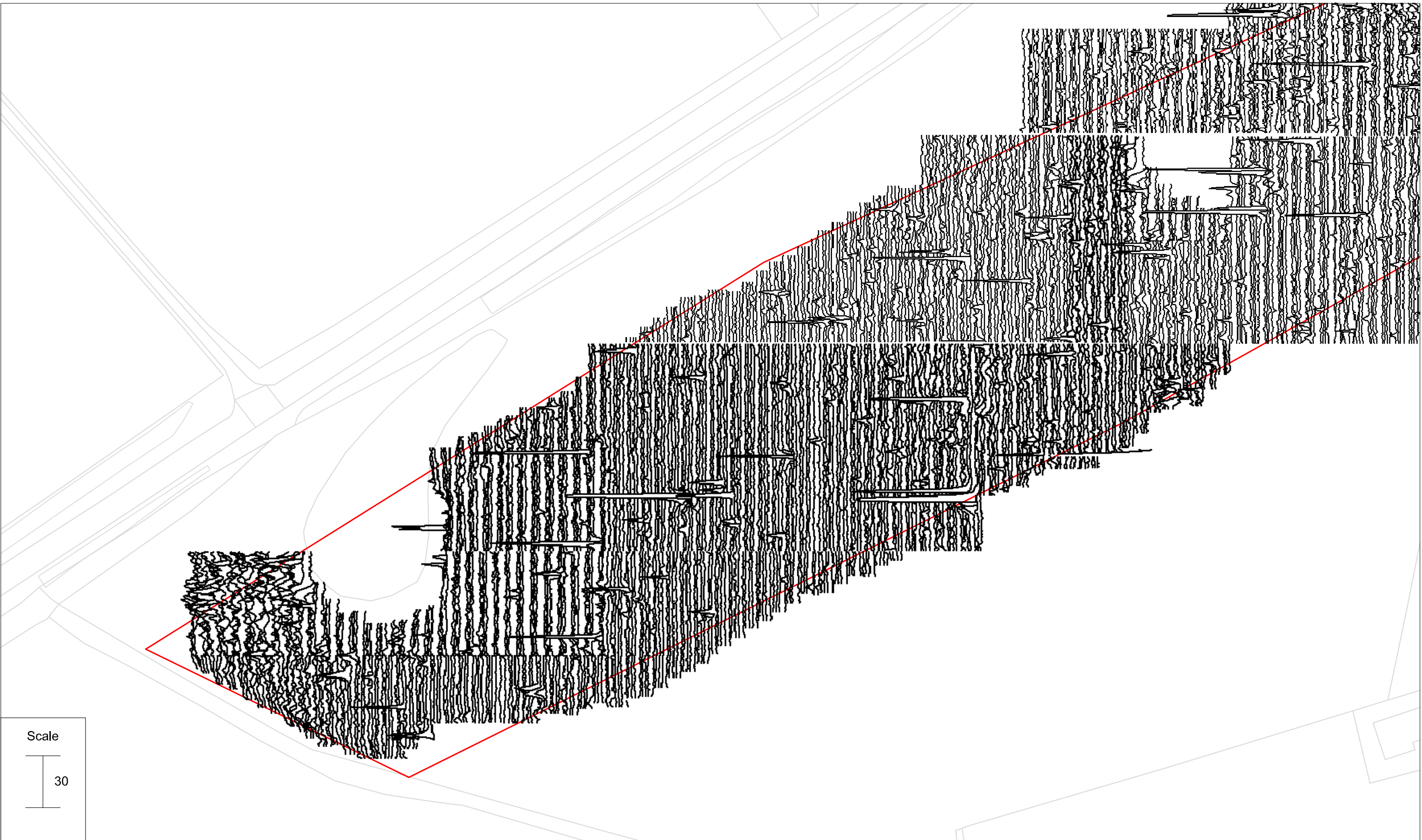
Minimally processed gradiometer survey results xy trace plot: parcel 10 west
