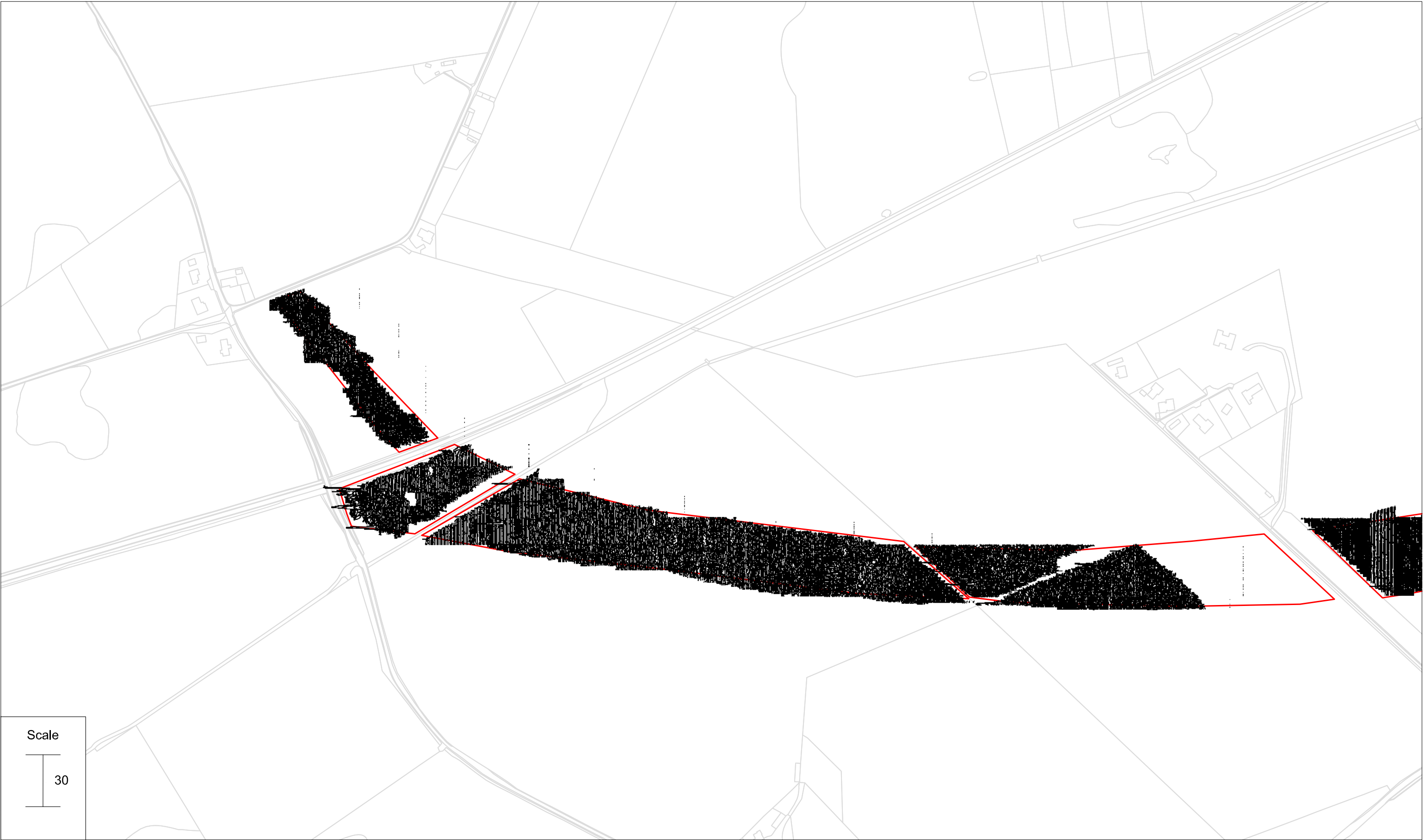
Minimally processed gradiometer survey results xy trace plot: parcel 12
