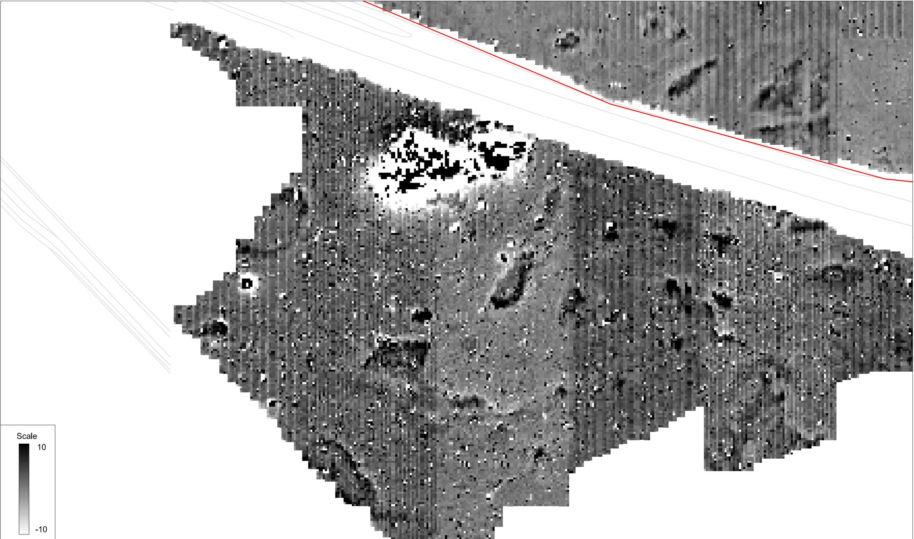
Unprocessed gradiometer survey results greyscale plot: parcel 15a west
