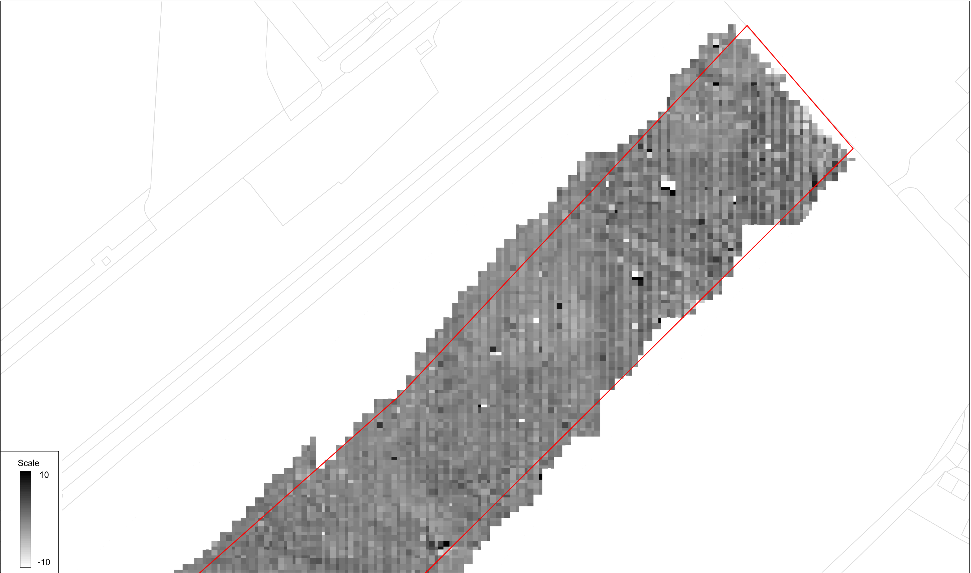
Unprocessed gradiometer survey results greyscale plot: parcel 8a east
