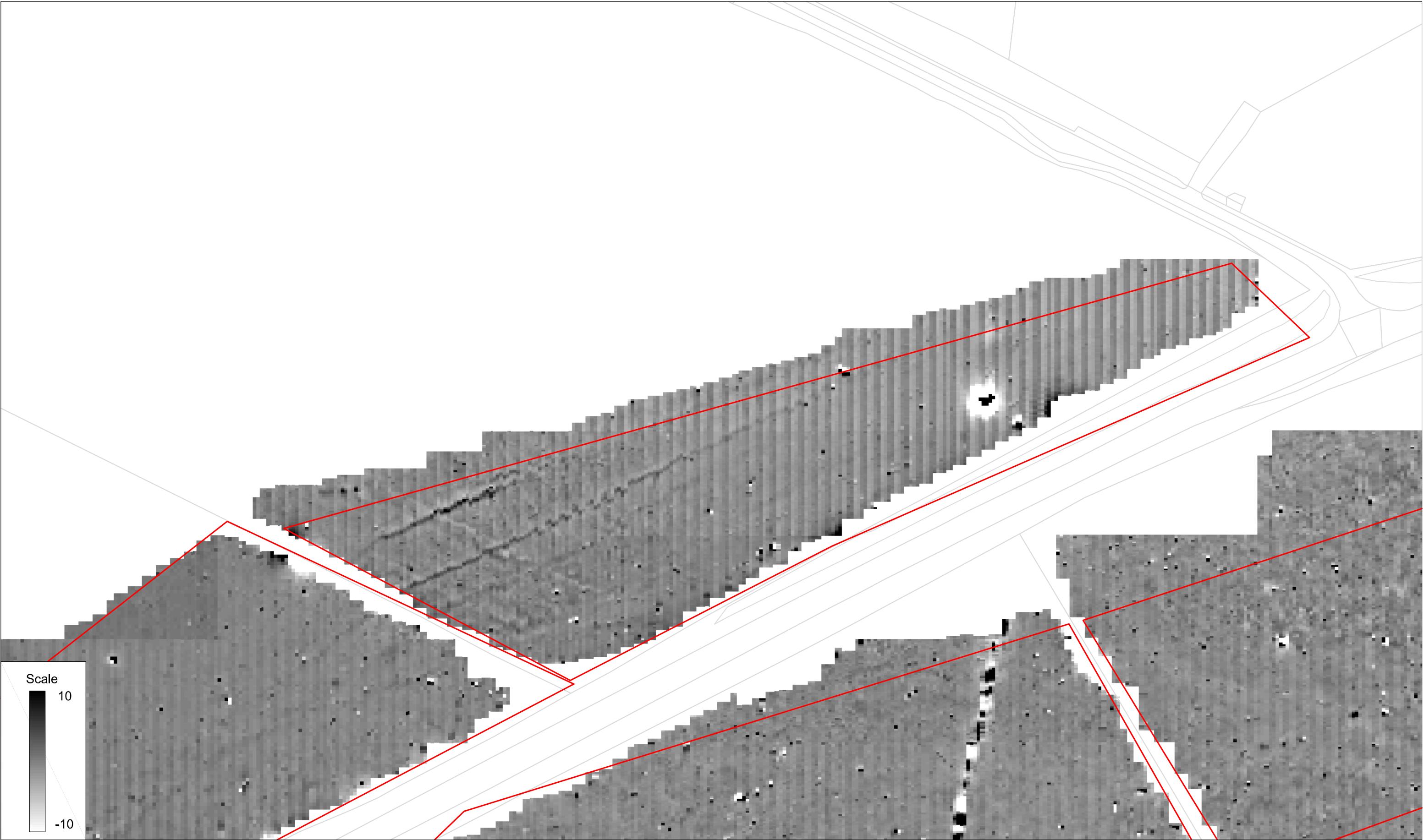
Unprocessed gradiometer survey results greyscale plot: parcel 17a
