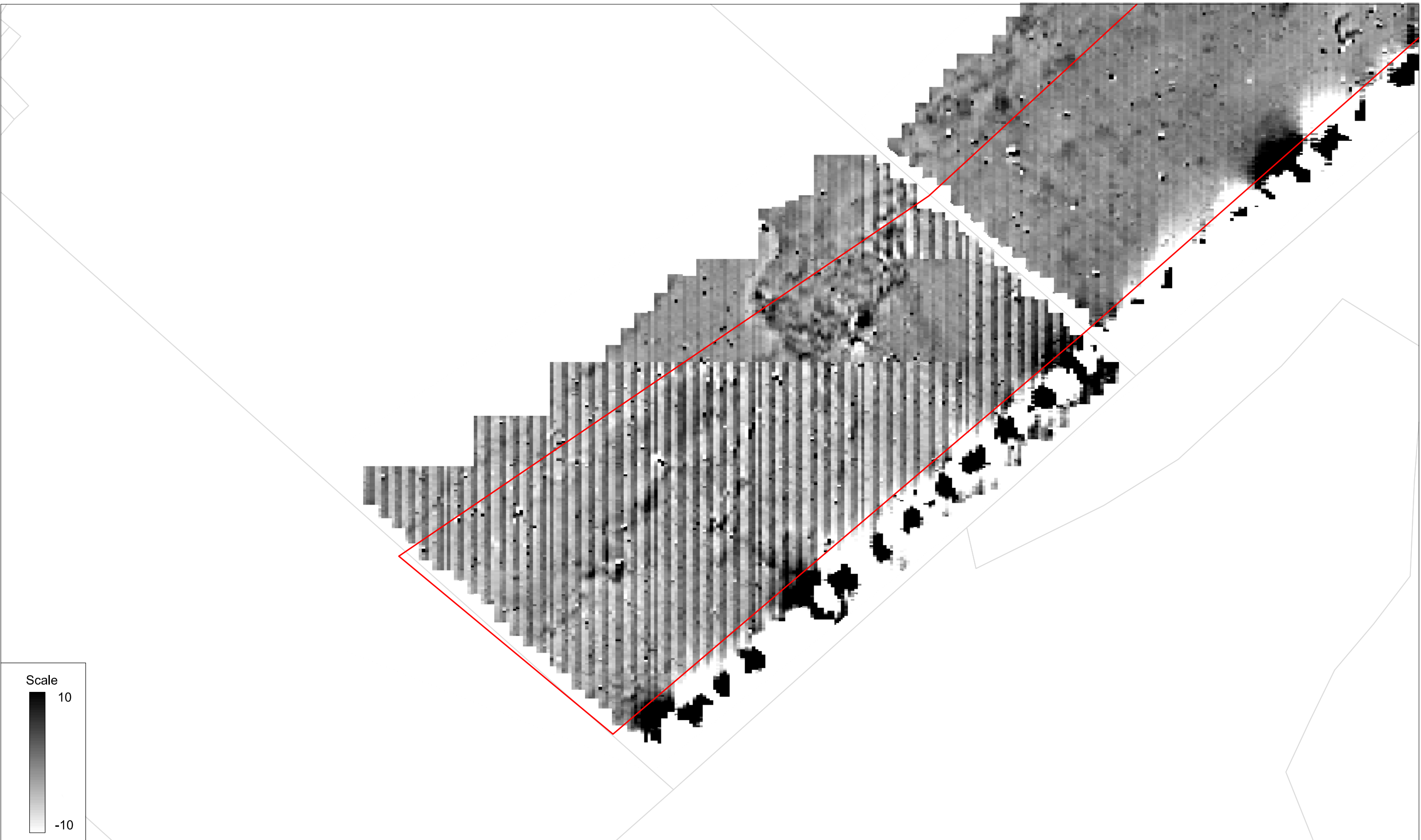
Unprocessed gradiometer survey results greyscale plot: parcel 14b
