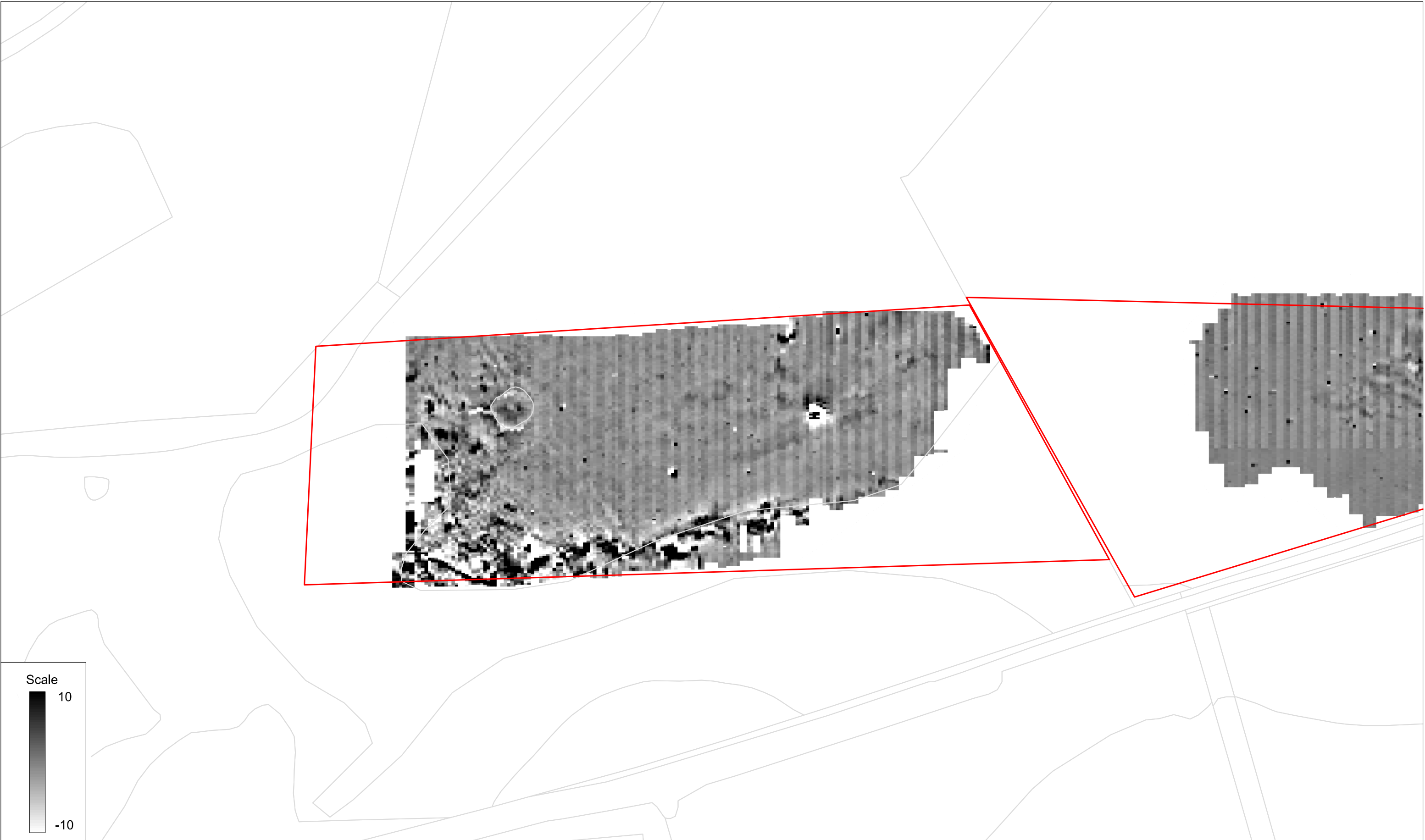
Unprocessed gradiometer survey results greyscale plot: parcel 11a
