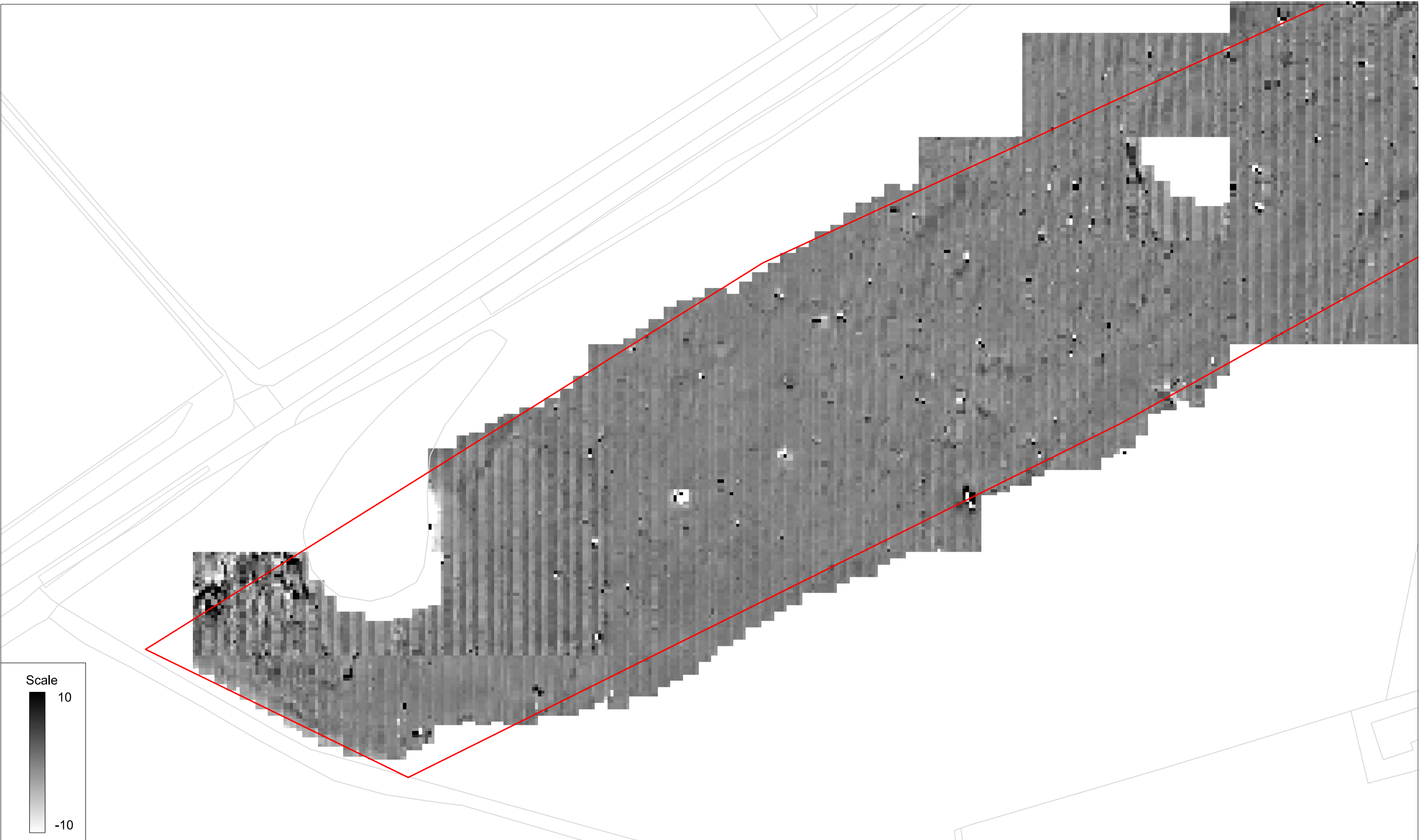
Unprocessed gradiometer survey results greyscale plot: parcel 10 west
