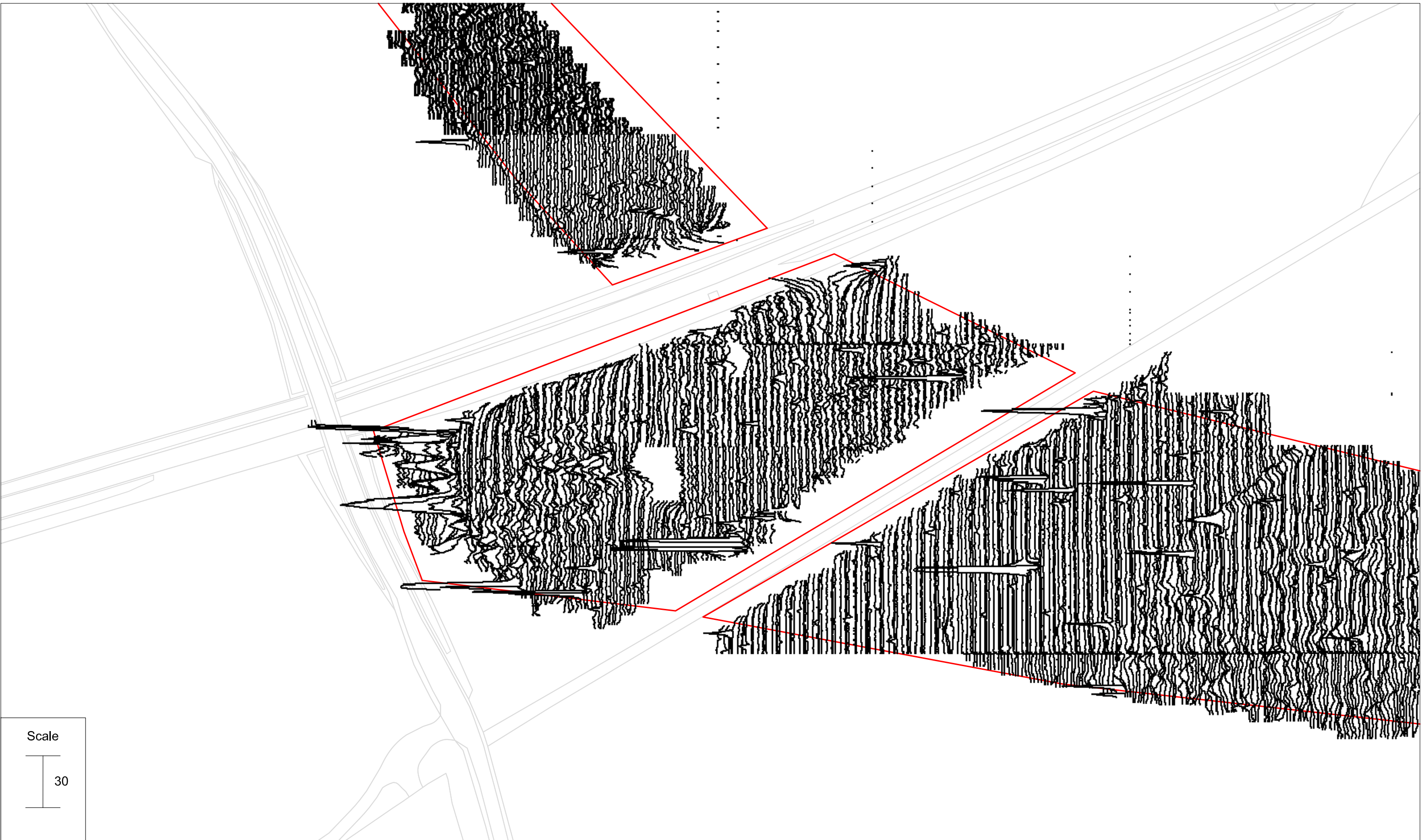
Minimally processed gradiometer survey results xy trace plot: parcel 12b
