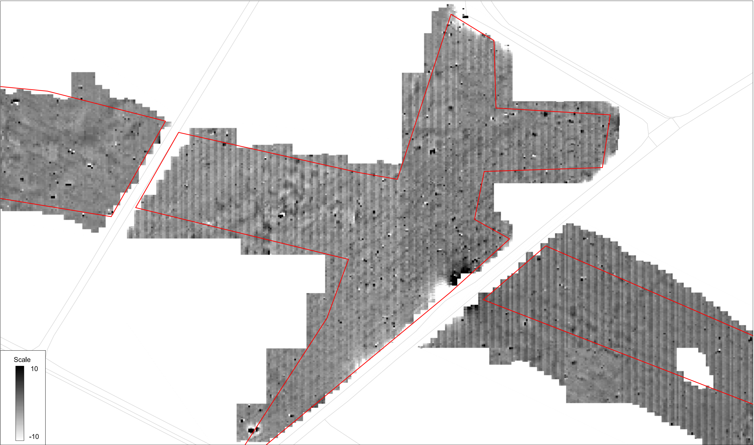
Unprocessed gradiometer survey results greyscale plot: parcel 15b
