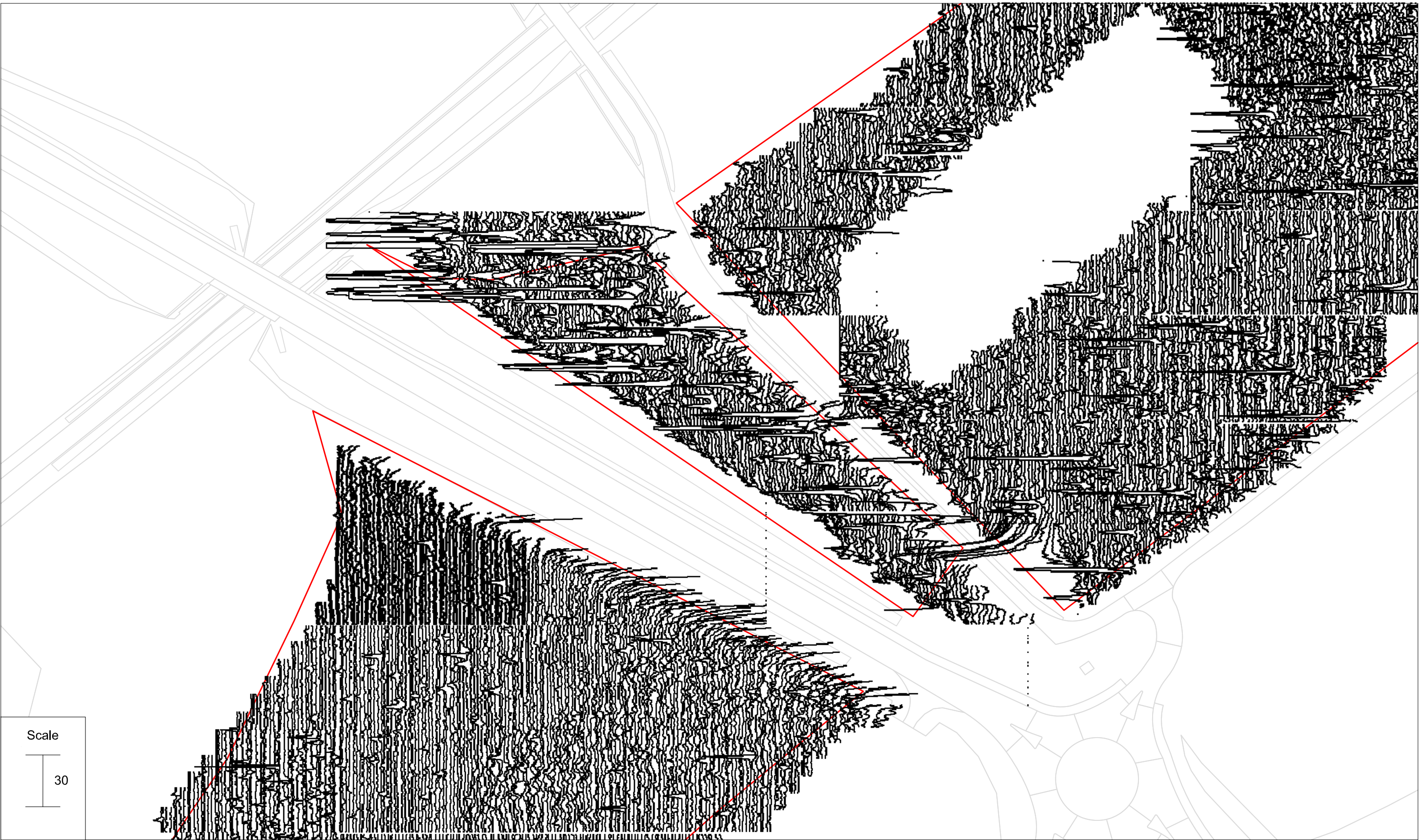
Minimally processed gradiometer survey results xy trace plot: parcel 8c, 8b and 8a
