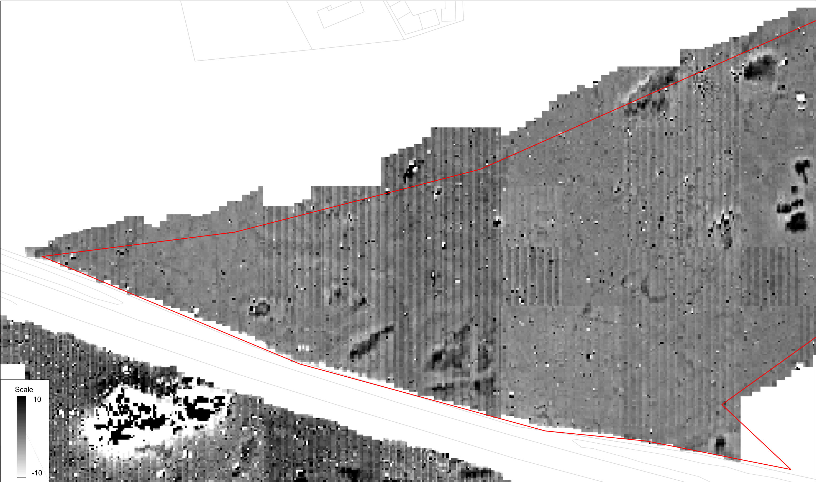
Unprocessed gradiometer survey results greyscale plot: parcel 15b west
