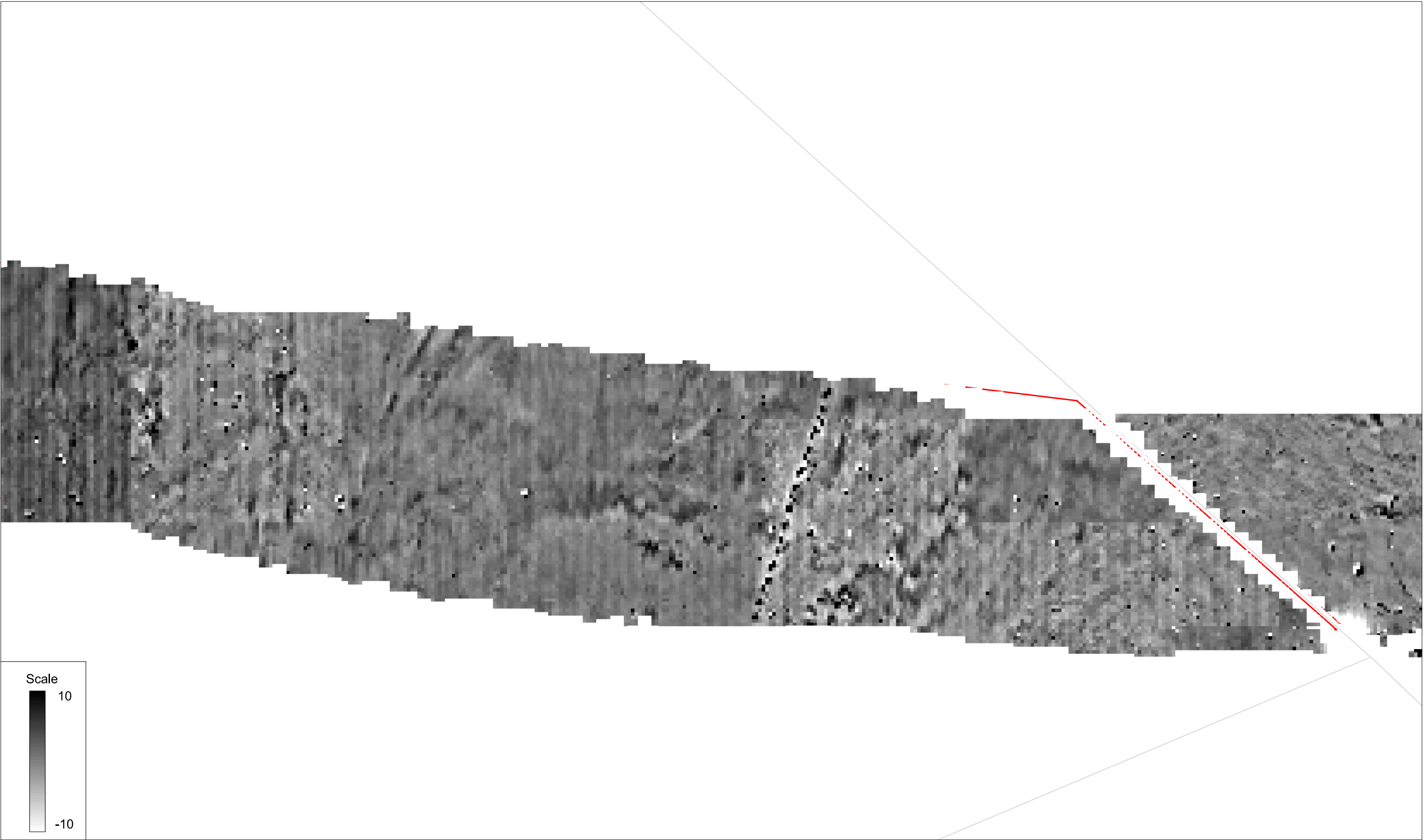
Unprocessed gradiometer survey results greyscale plot: parcel 12c east
