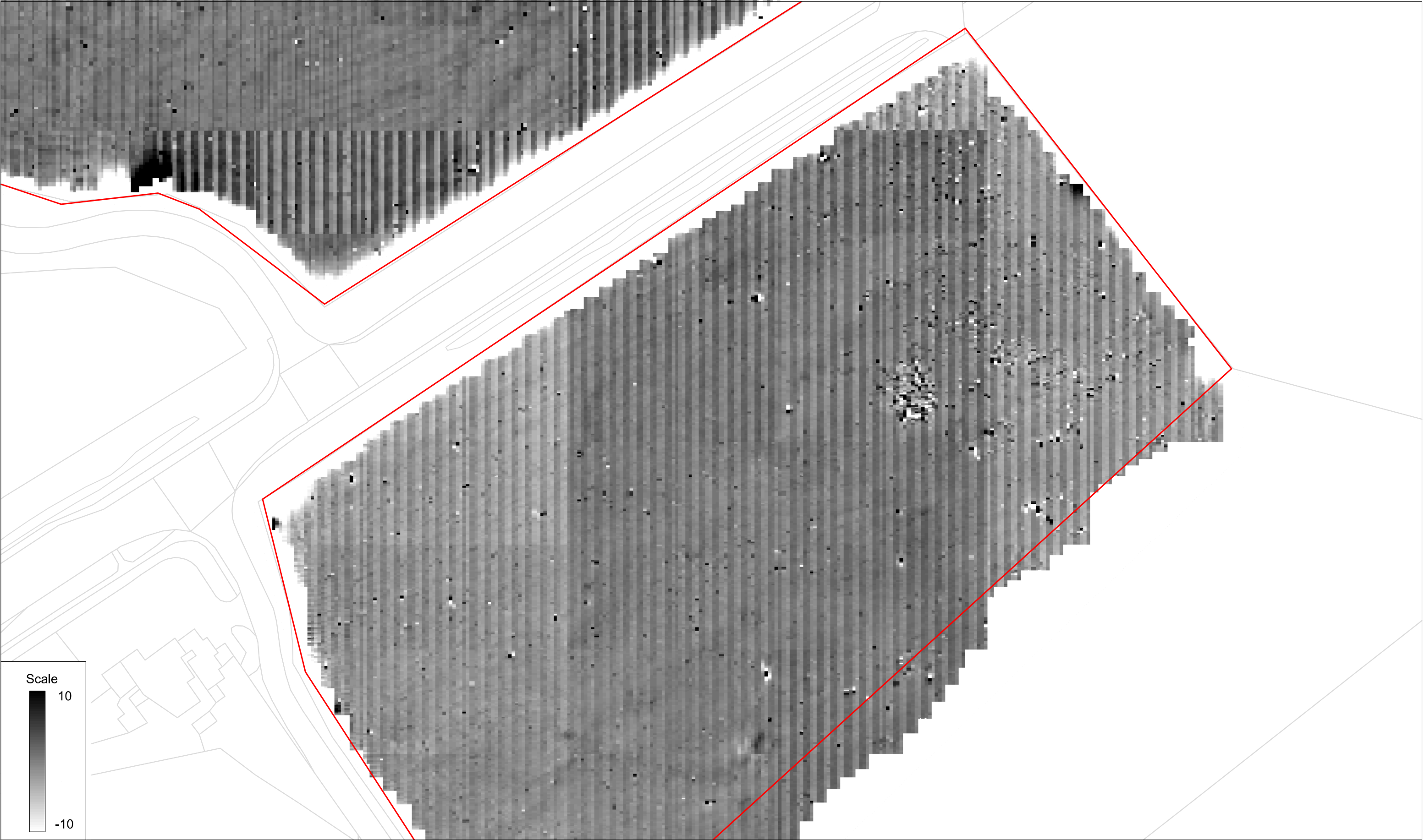
Unprocessed gradiometer survey results greyscale plot: parcel 9a north
