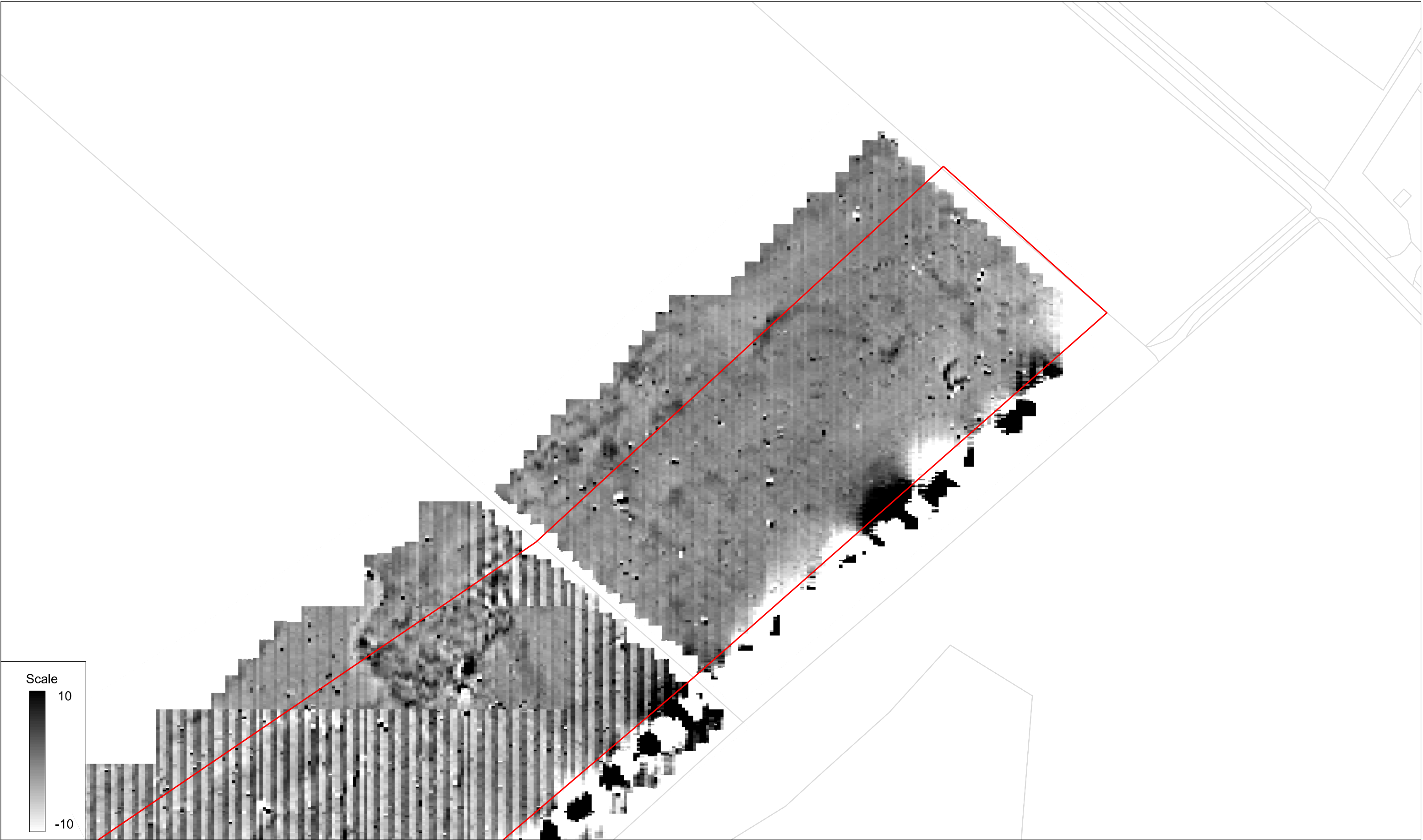
Unprocessed gradiometer survey results greyscale plot: parcel 14a
