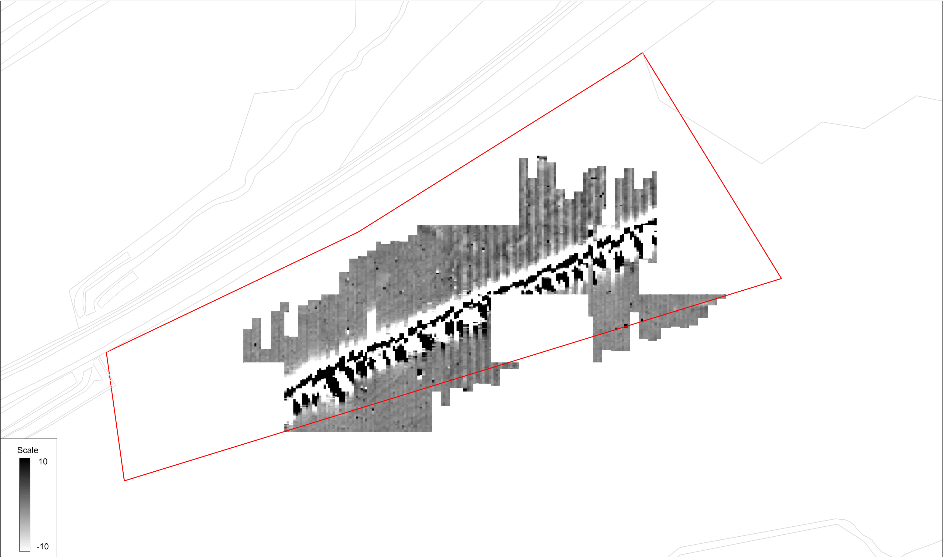
Unprocessed gradiometer survey results greyscale plot: parcel 1
