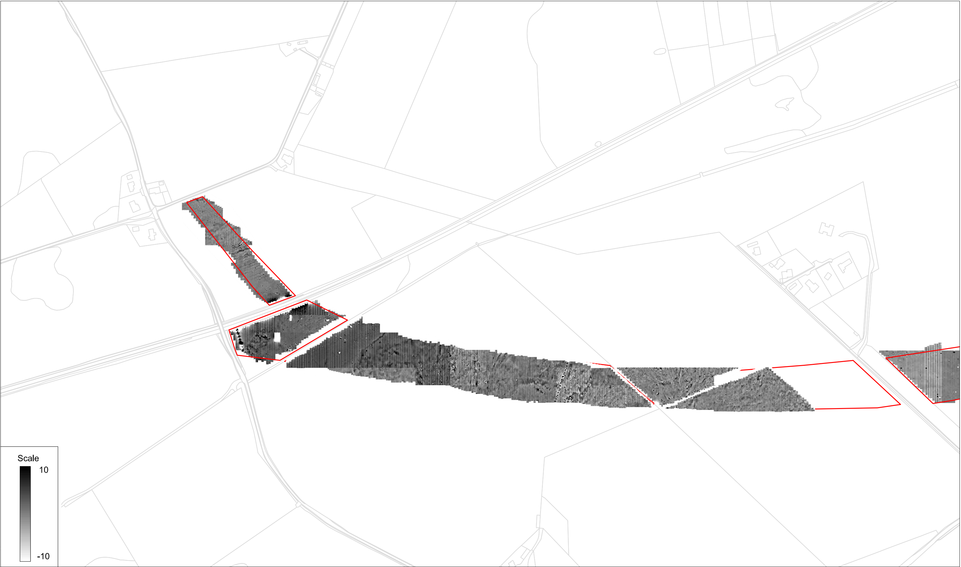
Unprocessed gradiometer survey results greyscale plot: parcel 12
