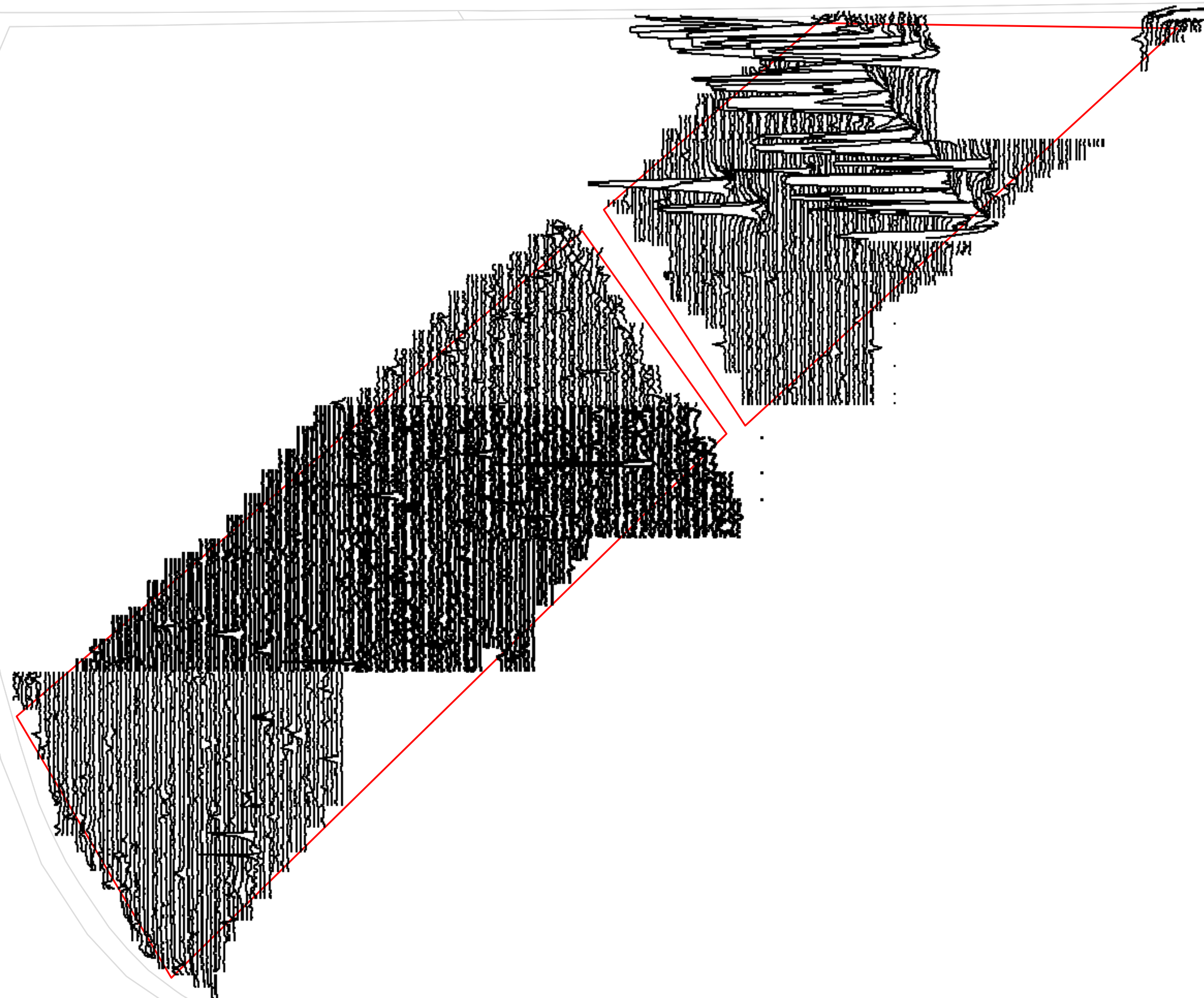
Minimally processed gradiometer survey results xy trace plot: parcel 7
