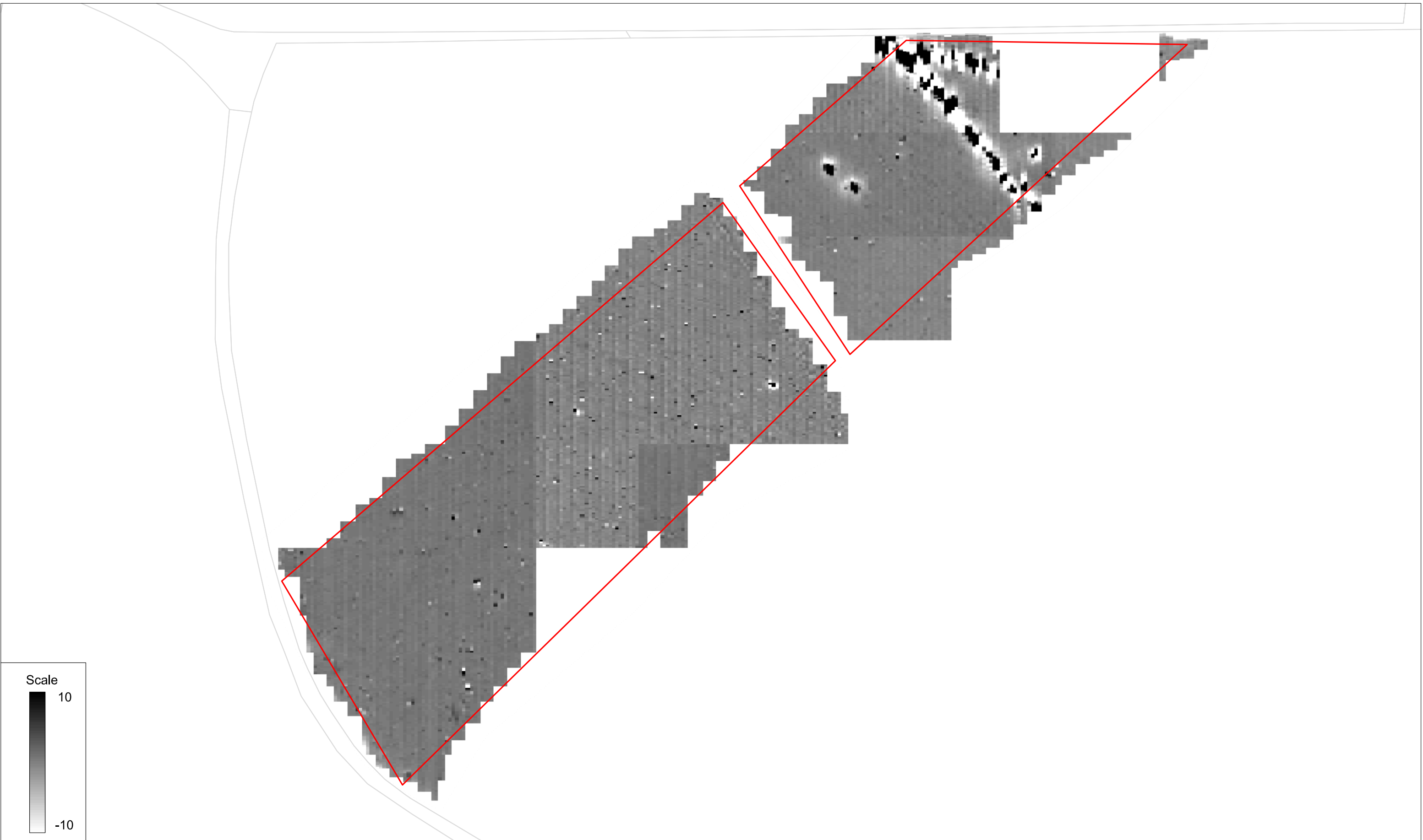
Unprocessed gradiometer survey results greyscale plot: parcel 7
