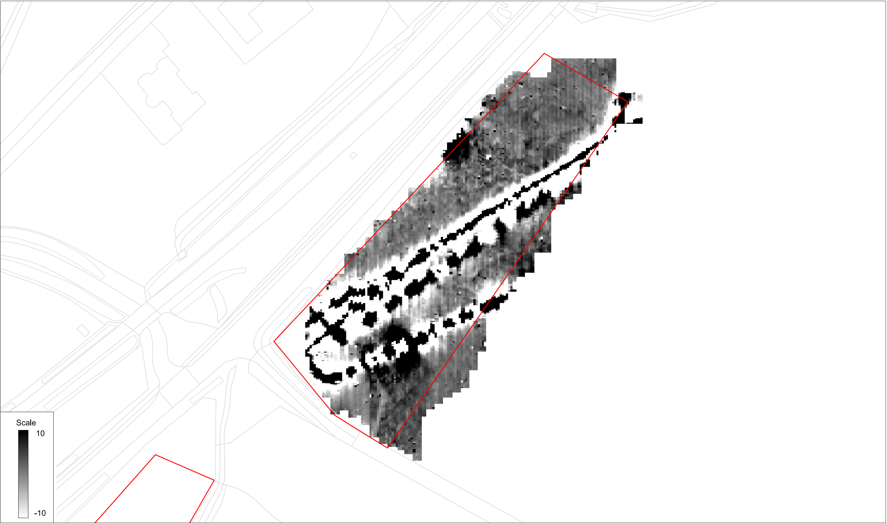
Unprocessed gradiometer survey results greyscale plot: parcel 3
