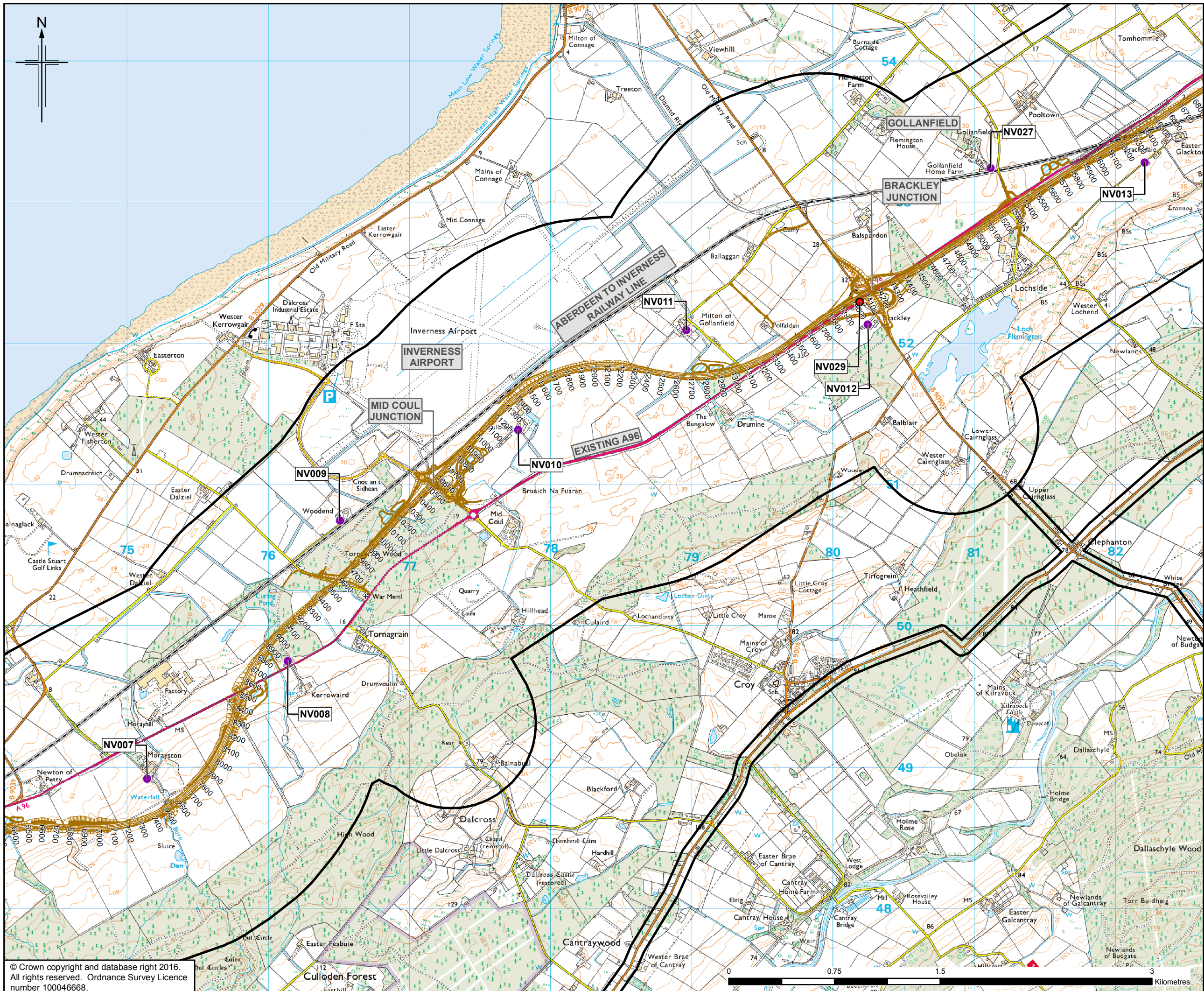
Drawing title Figure 8.2b Environmental Statement Baseline Noise Monitoring Locations and Sample Receptors
