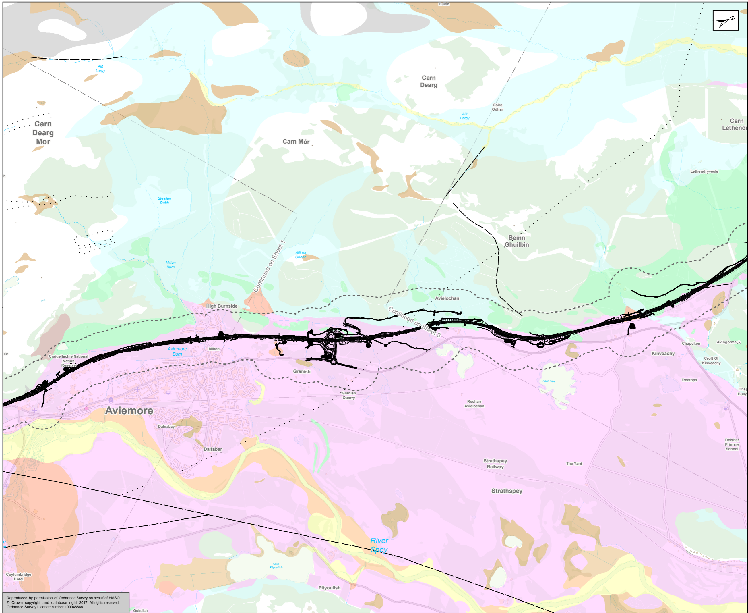
Figure 10.2 Superficial Geology Sheet 2 of 5
