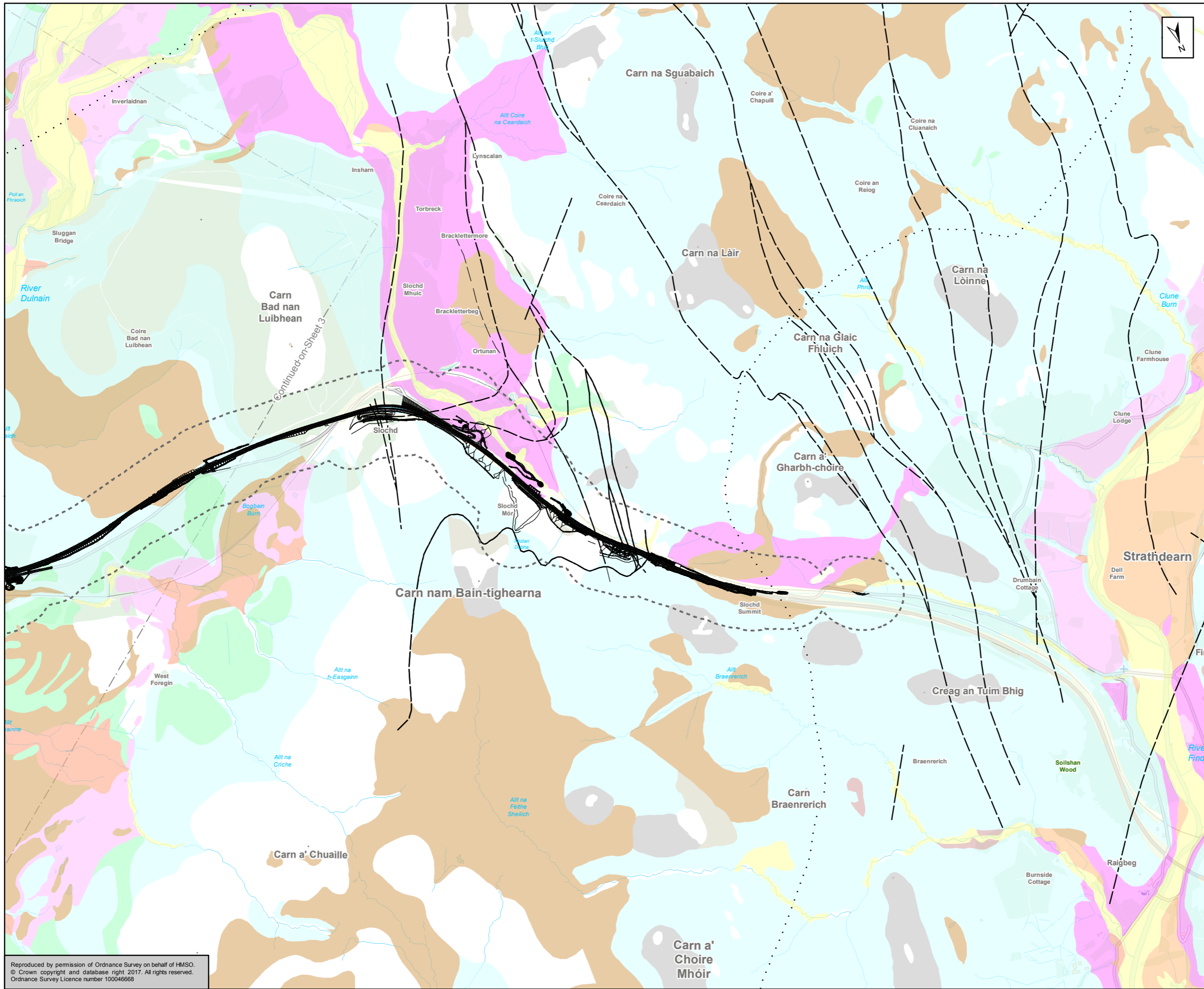
Figure 10.2 Superficial Geology Sheet 4 of 5
