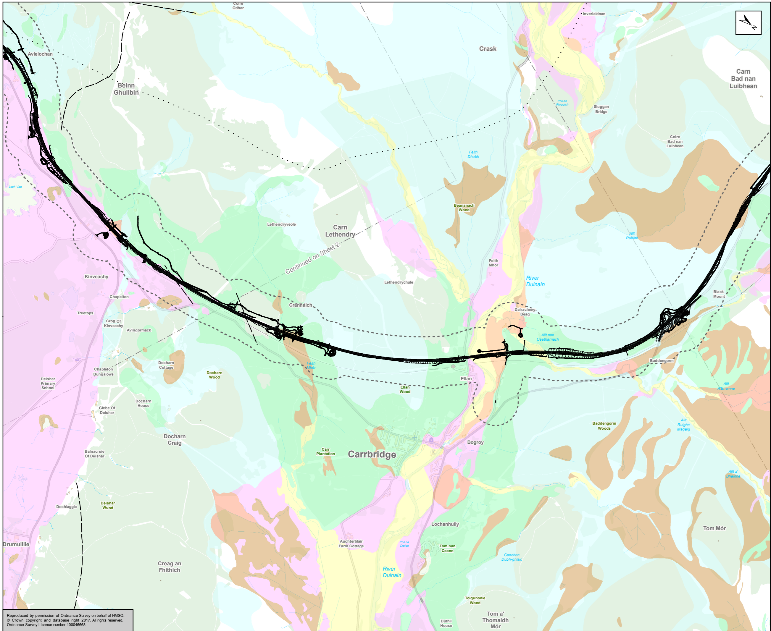
Figure 10.2 Superficial Geology Sheet 3 of 5
