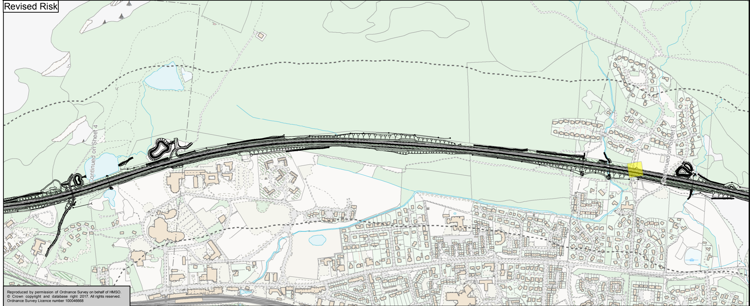
Figure A10.2.4 Initial Risk and Revised Risk Areas Sheet 5 of 17
