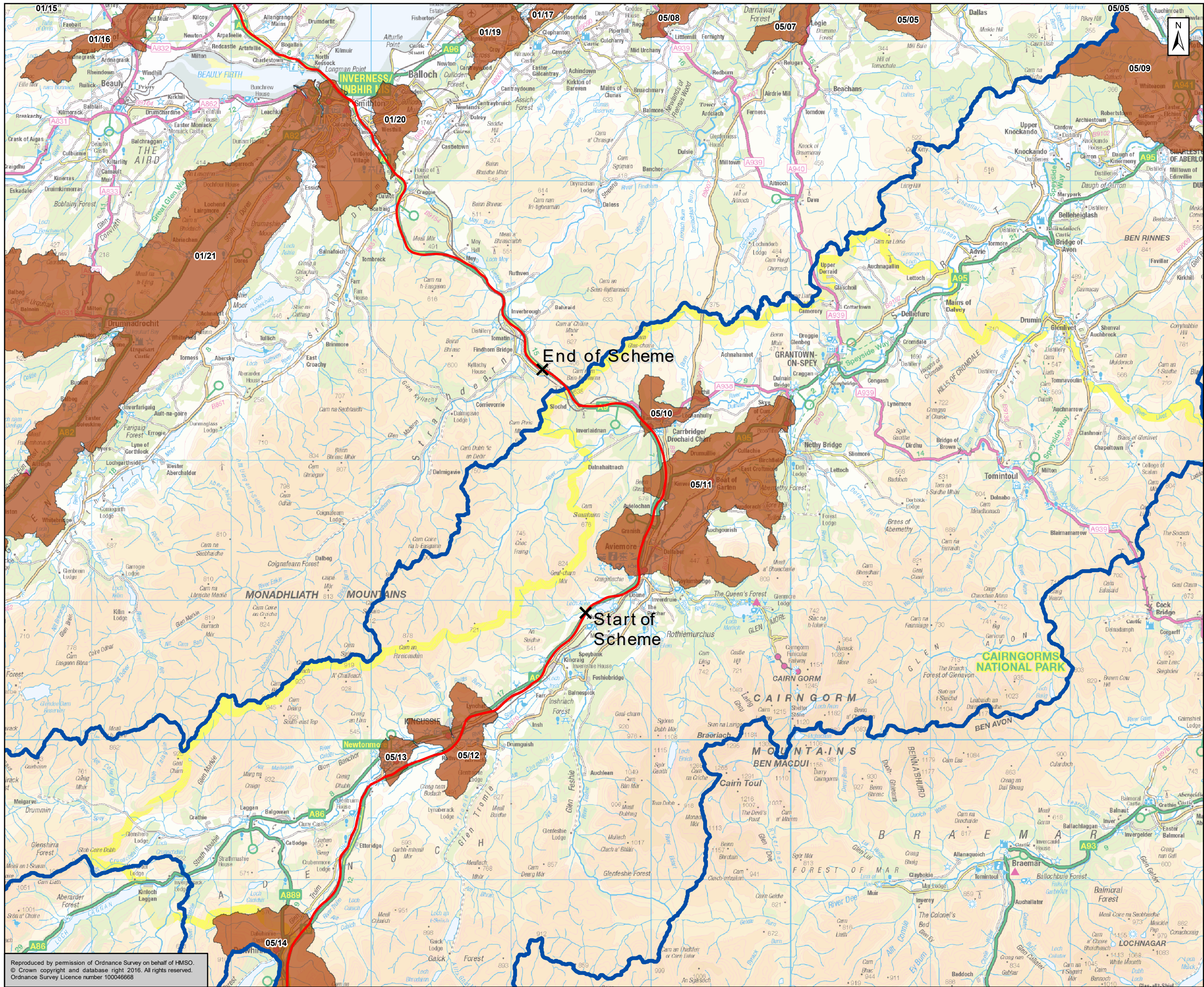
Figure A11.3.3 River Spey Catchment & Potentially Vulnerable Areas Sheet 1 of 1
