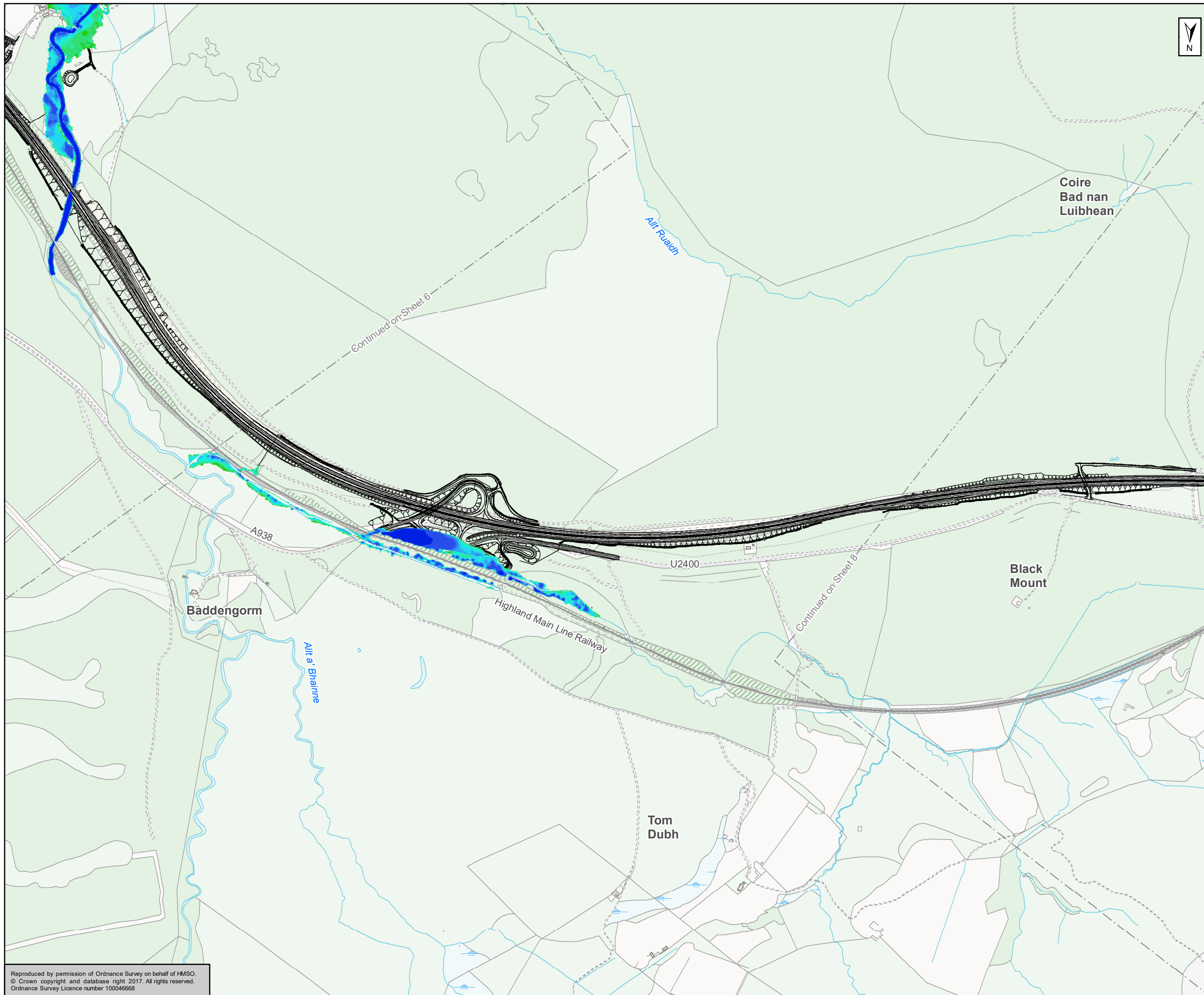
Figure A11.3.8 AMJV 0.5% Baseline Sheet 7 of 9
