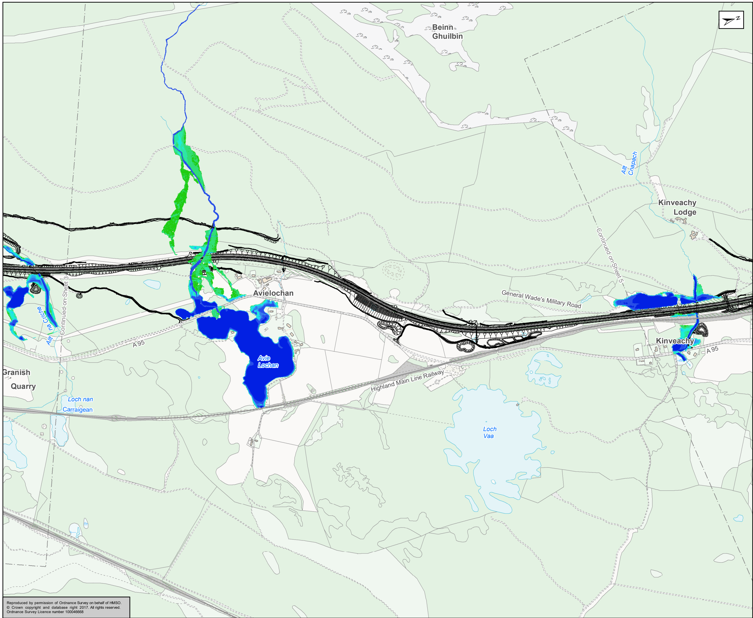
Figure A11.3.8 AMJV 0.5% Baseline Sheet 4 of 9
