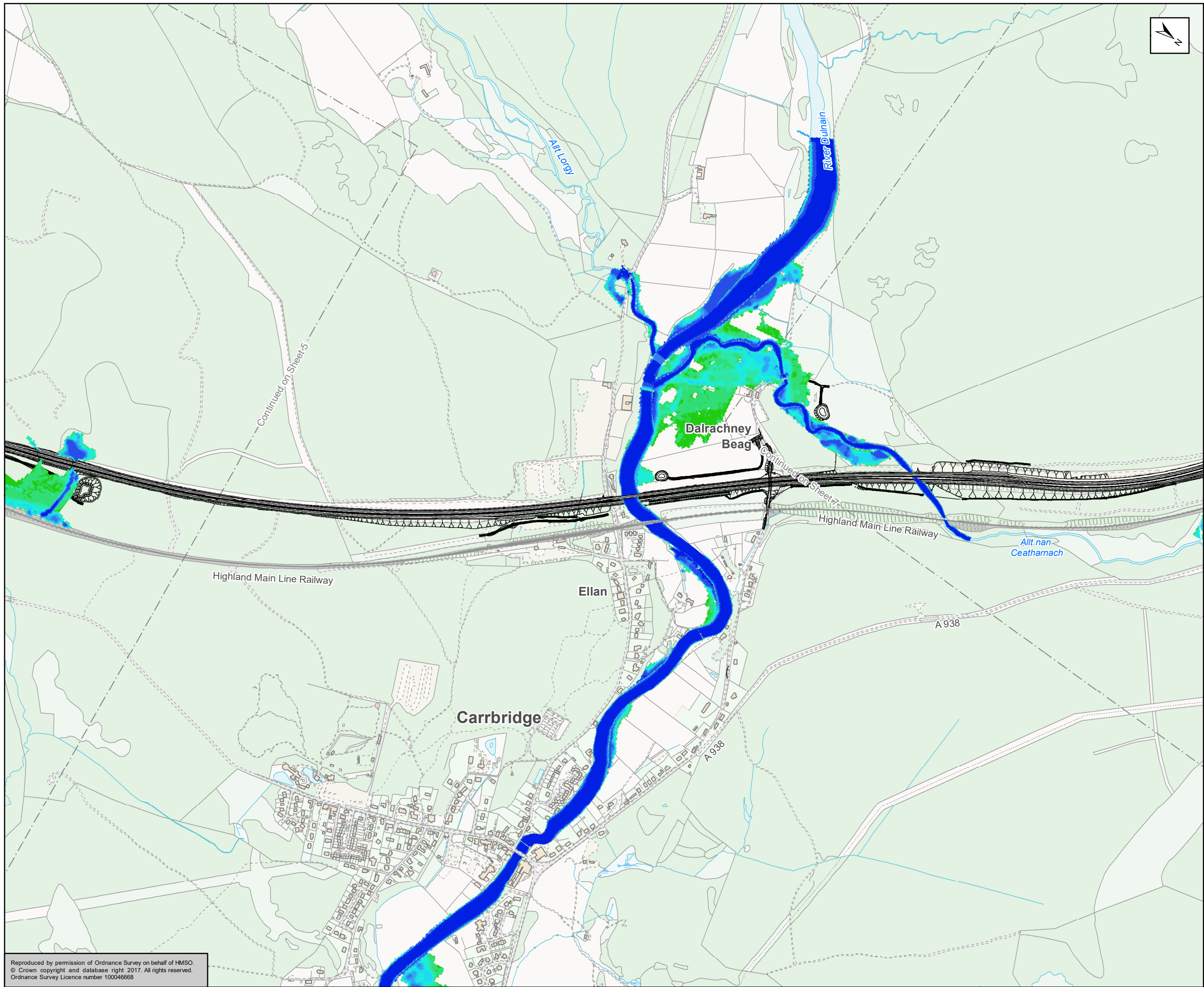
Figure A11.3.8 AMJV 0.5% Baseline Sheet 6 of 9
