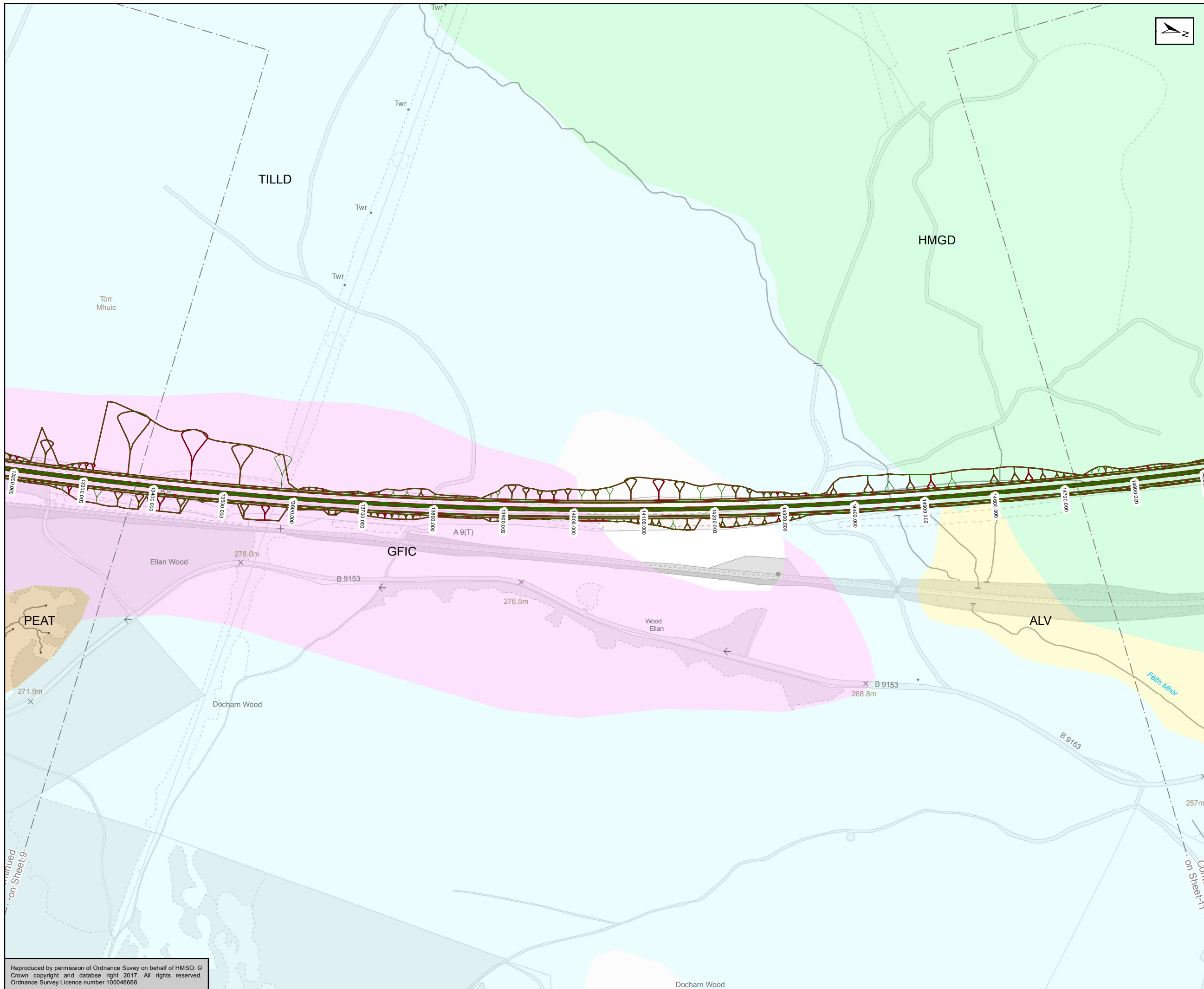
Figure 5.24j Mainline Alignment Option 2 Superficial Geology Sheet 10 of 17
