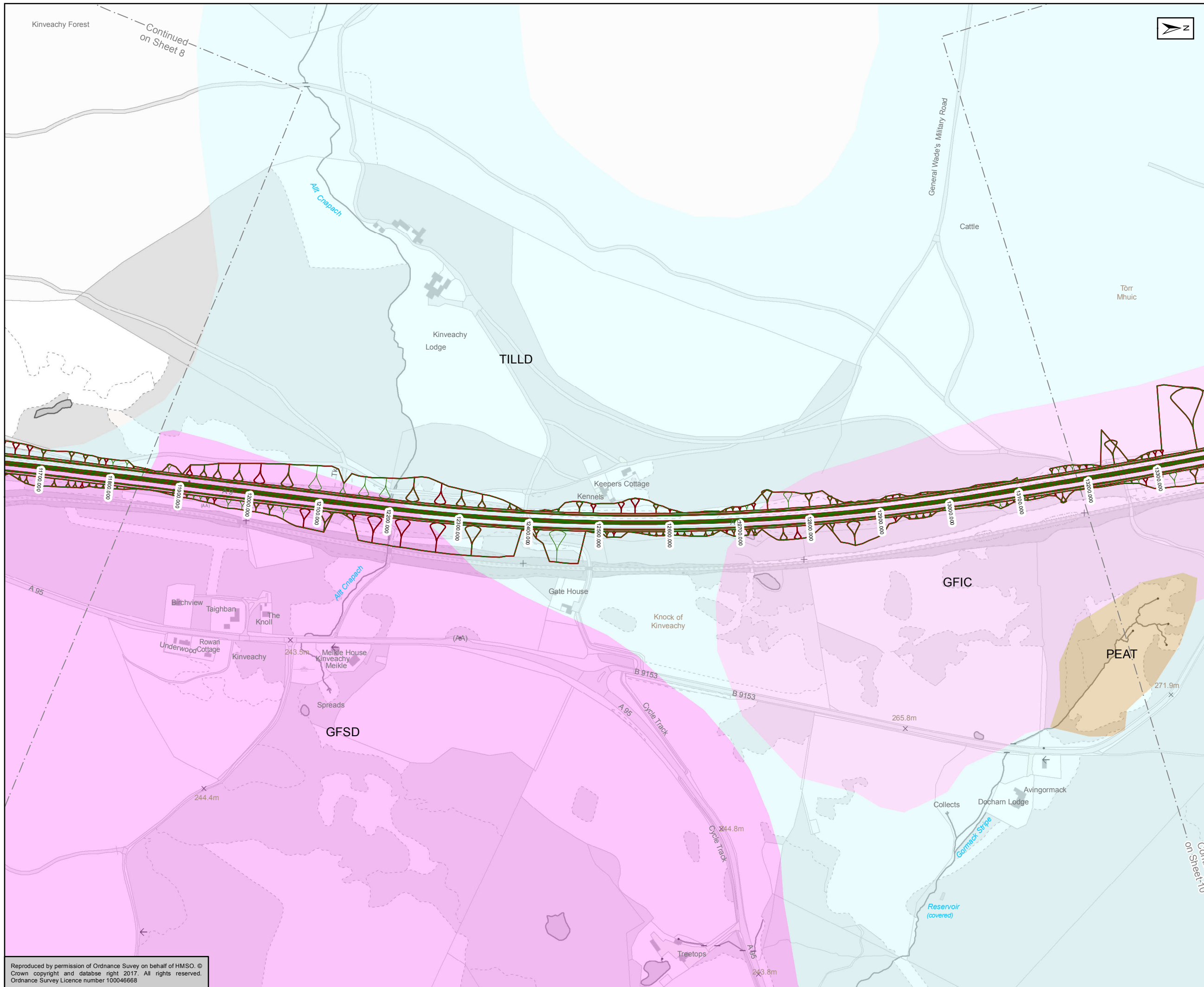
Figure 5.24i Mainline Alignment Option 2 Superficial Geology Sheet 9 of 17
