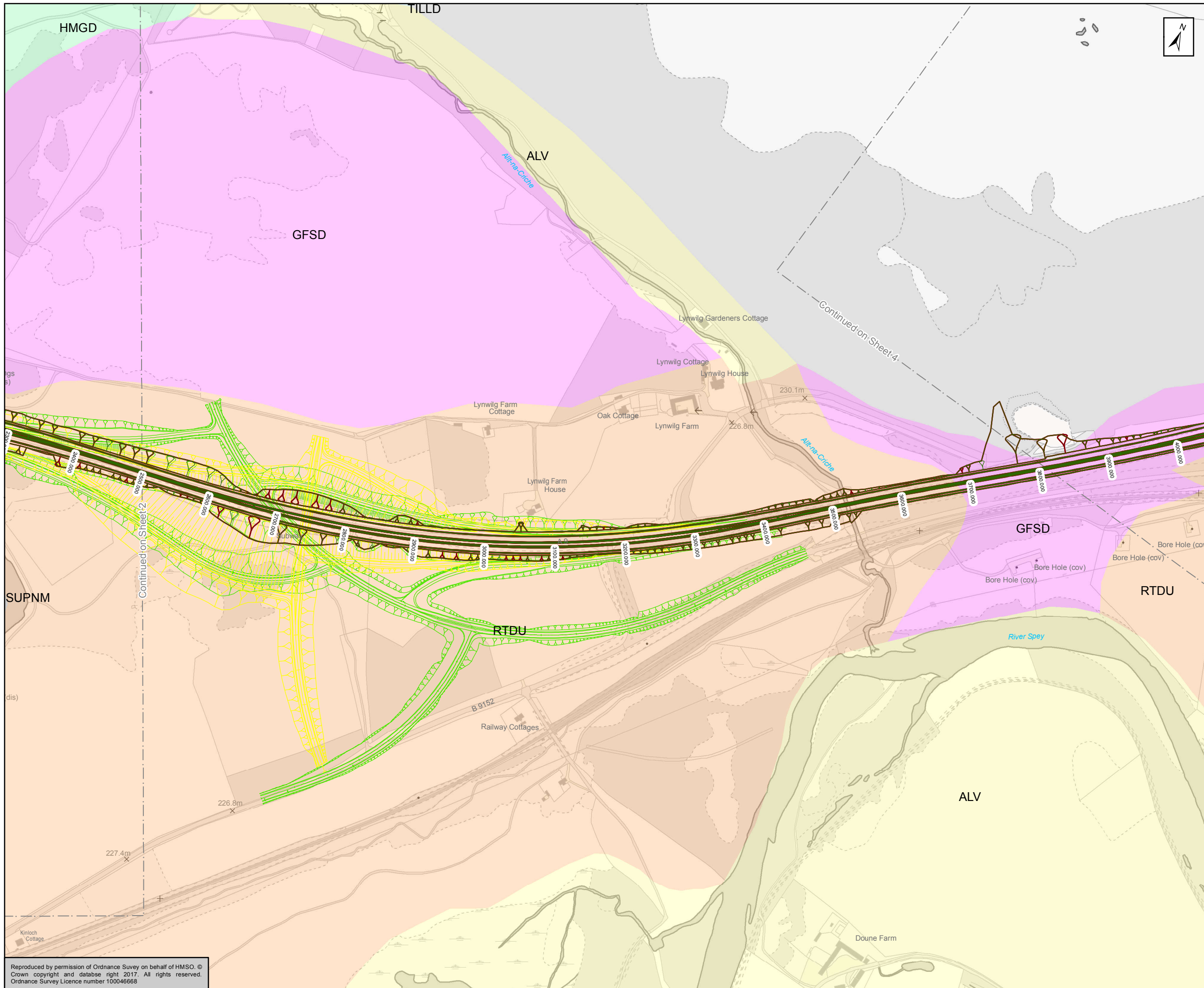
Figure 5.24c Mainline Alignment Option 2 Superficial Geology Sheet 3 of 17
