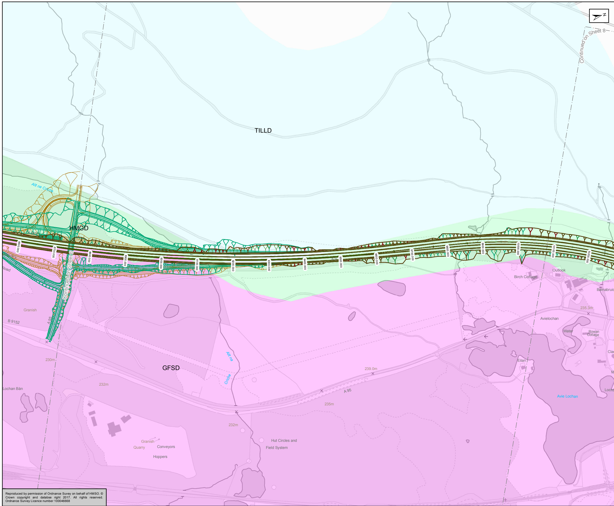
Figure 5.24g Mainline Alignment Option 2 Superficial Geology Sheet 7 of 17
