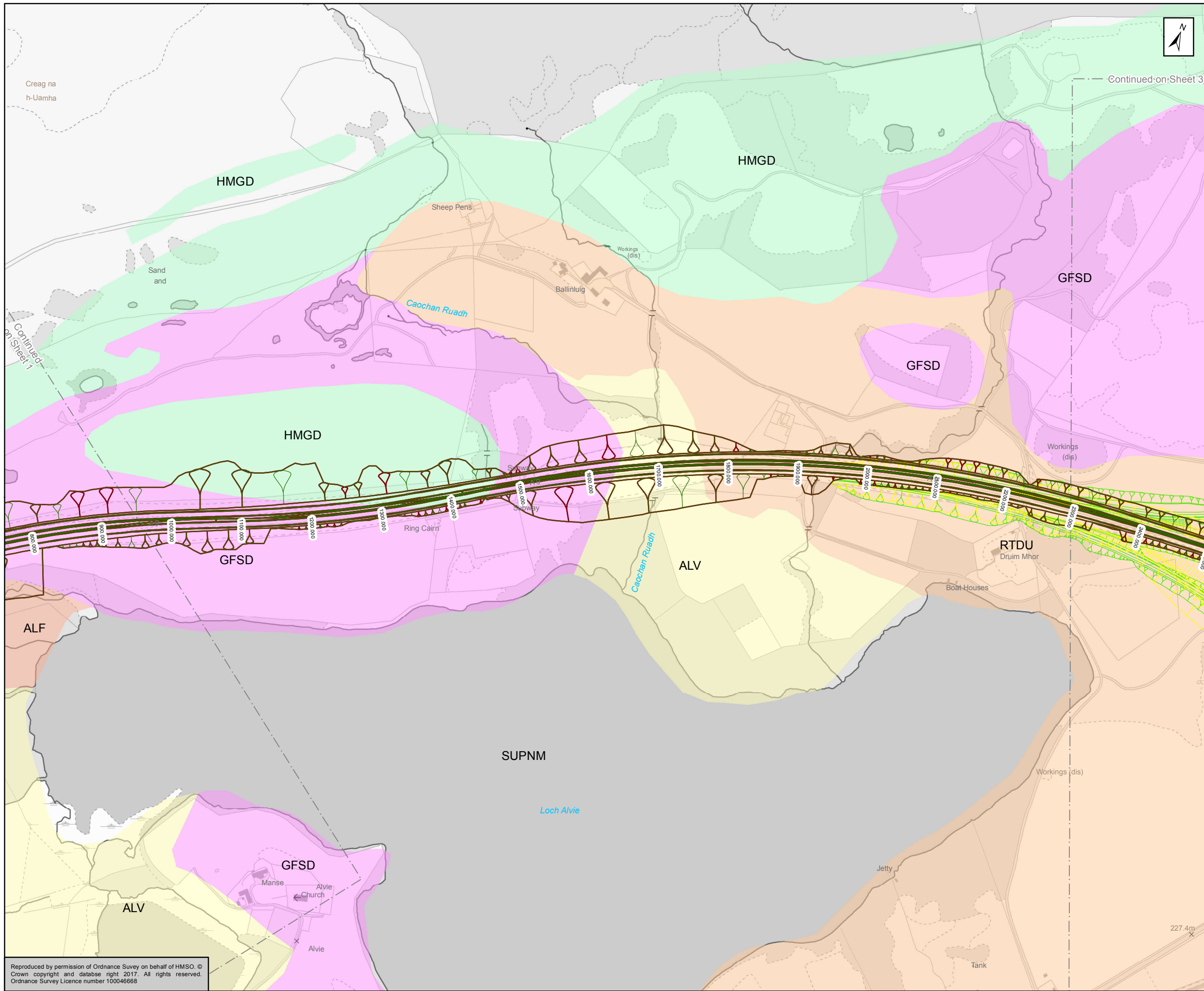
Figure 5.24b Mainline Alignment Option 2 Superficial Geology Sheet 2 of 17
