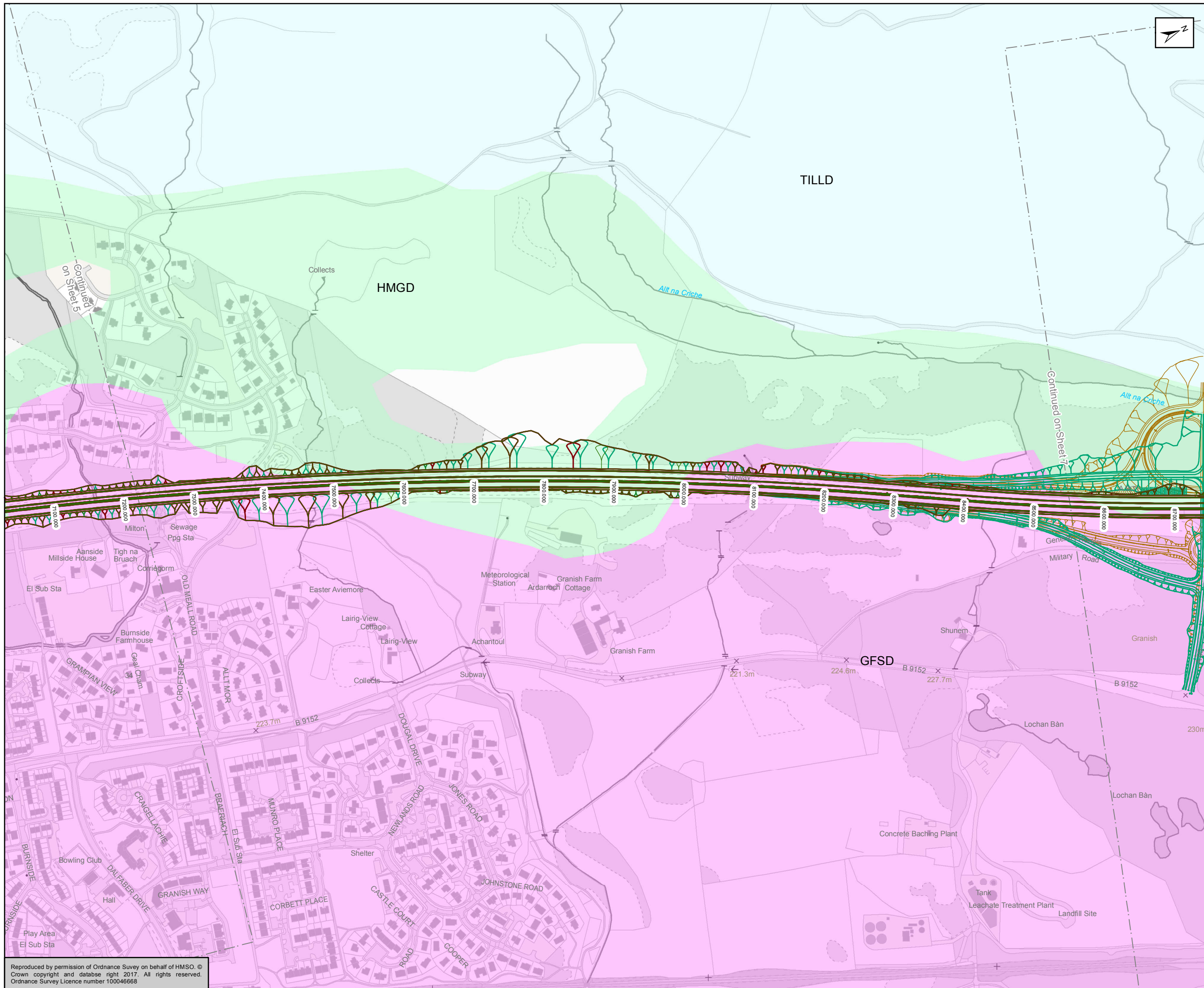
Figure 5.24f Mainline Alignment Option 2 Superficial Geology Sheet 6 of 17
