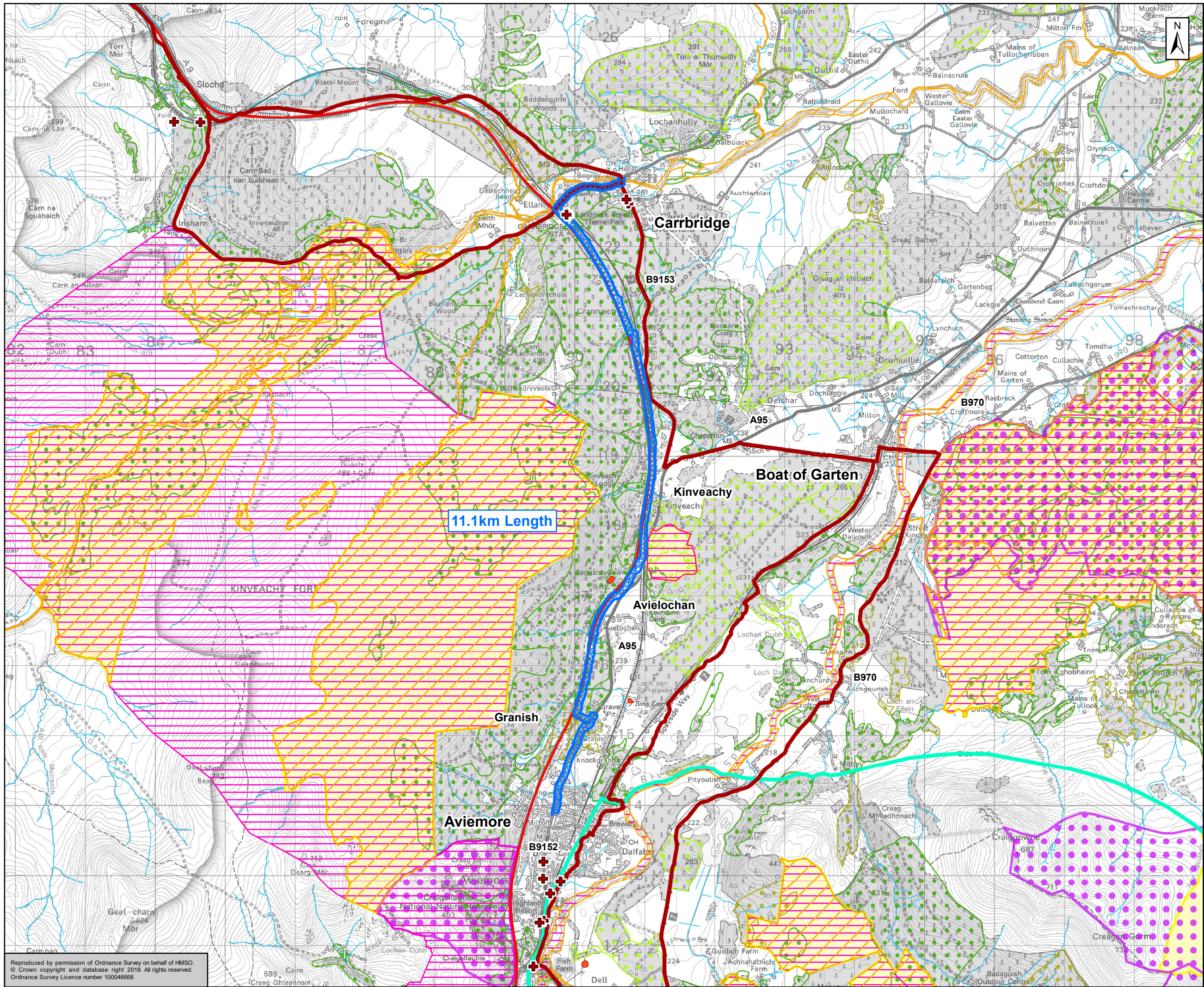
Figure 2.1 Identified Corridor Option 1 Segregated NMU Sheet 1 of 1
